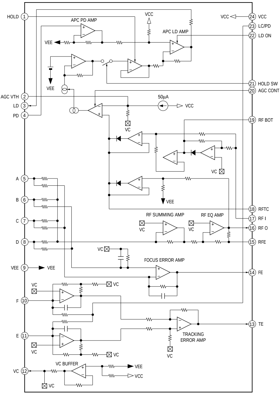
IC103 CXA2568M-T6
