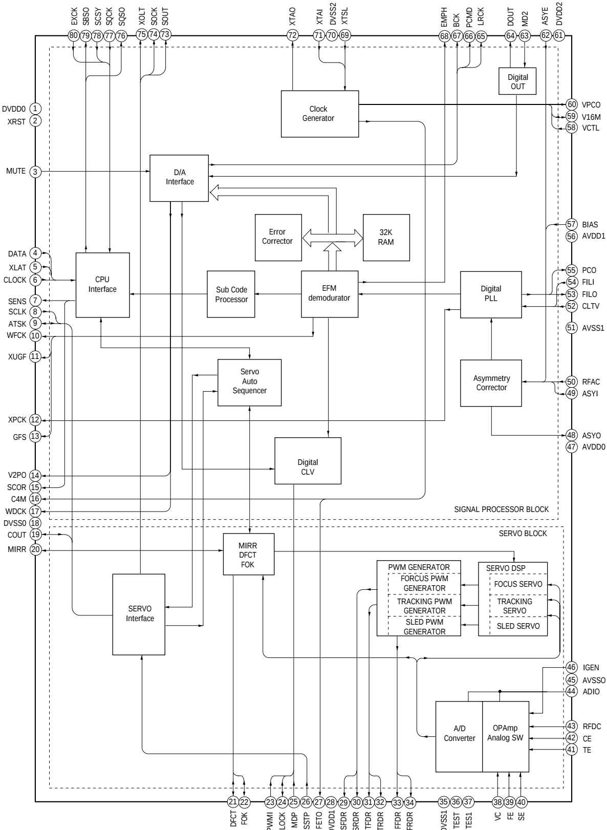
IC101 CDX2585Q
