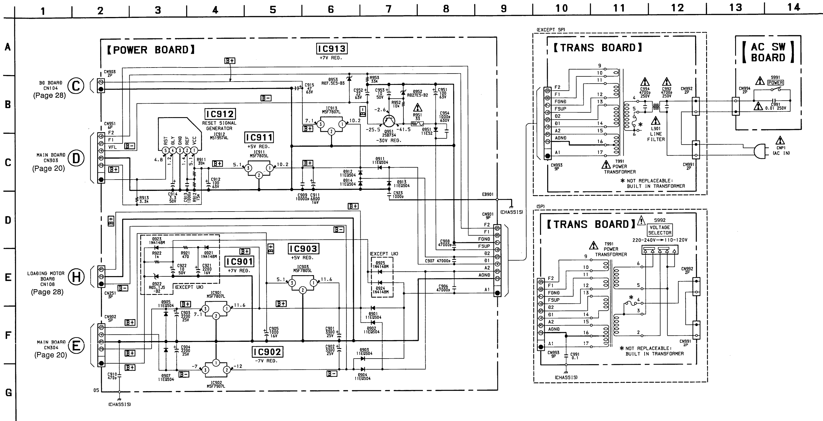
6-7. SCHEMATIC DIAGRAM – POWER Section – • See page 45 for IC Block Diagrams.
