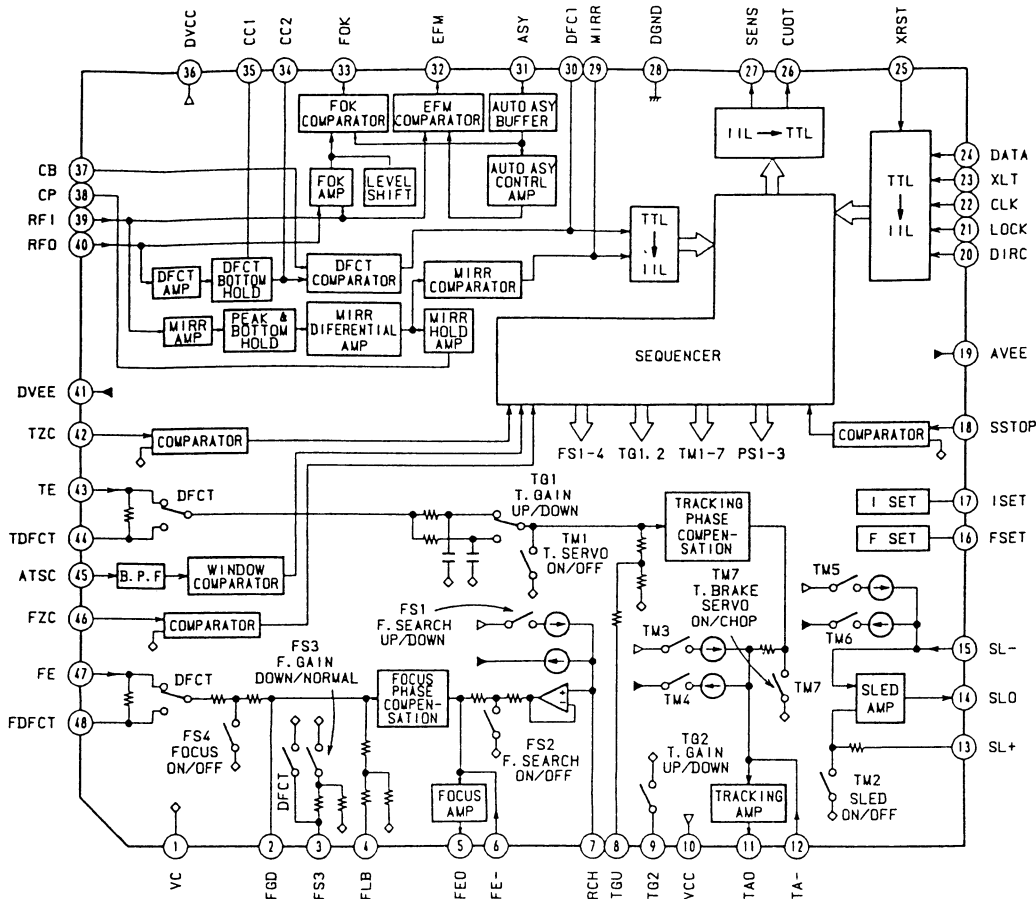
IC201 CXD2500AQ
