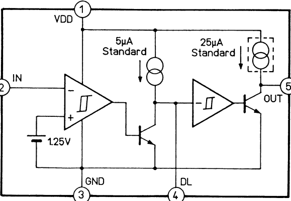
IC306 M51957AL
