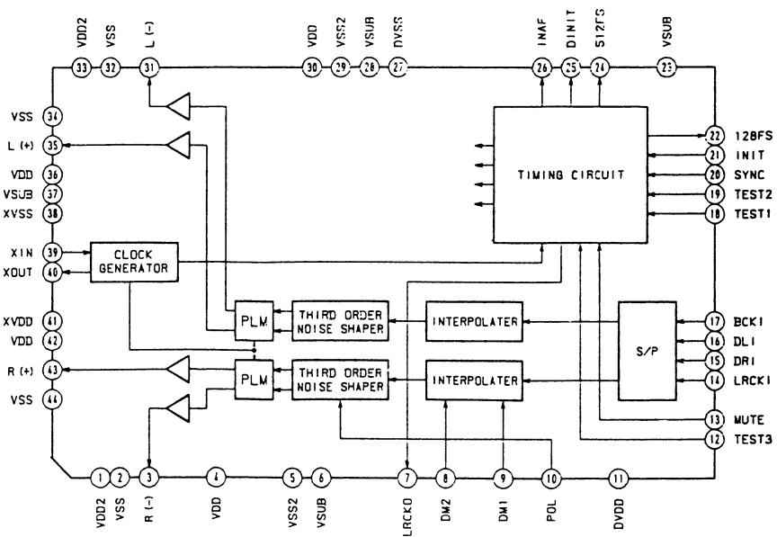
IC604 CXD1244S
