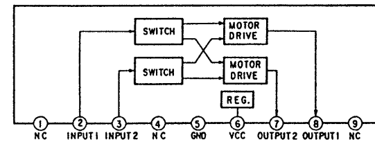
IC303 BA6208
