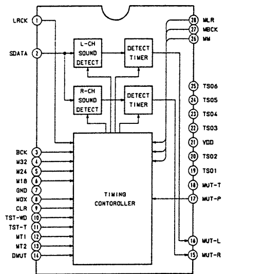
IC203 CXD2553S
