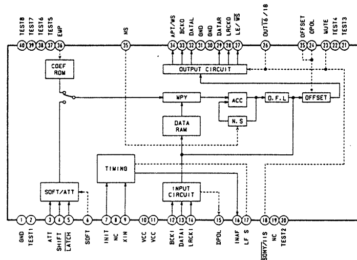
IC202 CXD1244S
