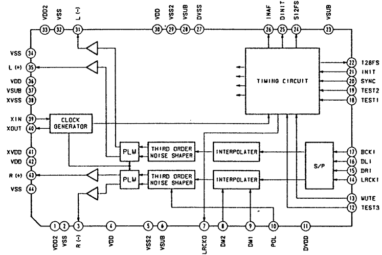
IC202 CXD1244S
