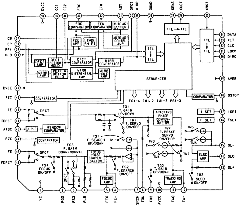
IC401 CXD2552Q
