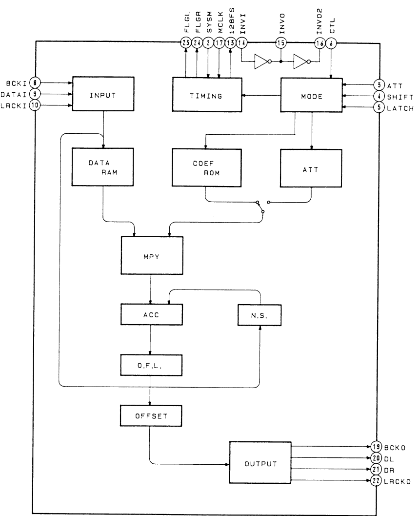
IC603 CXD2560M
