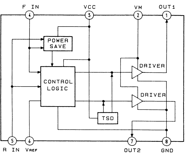
IC102 BA6297FP
