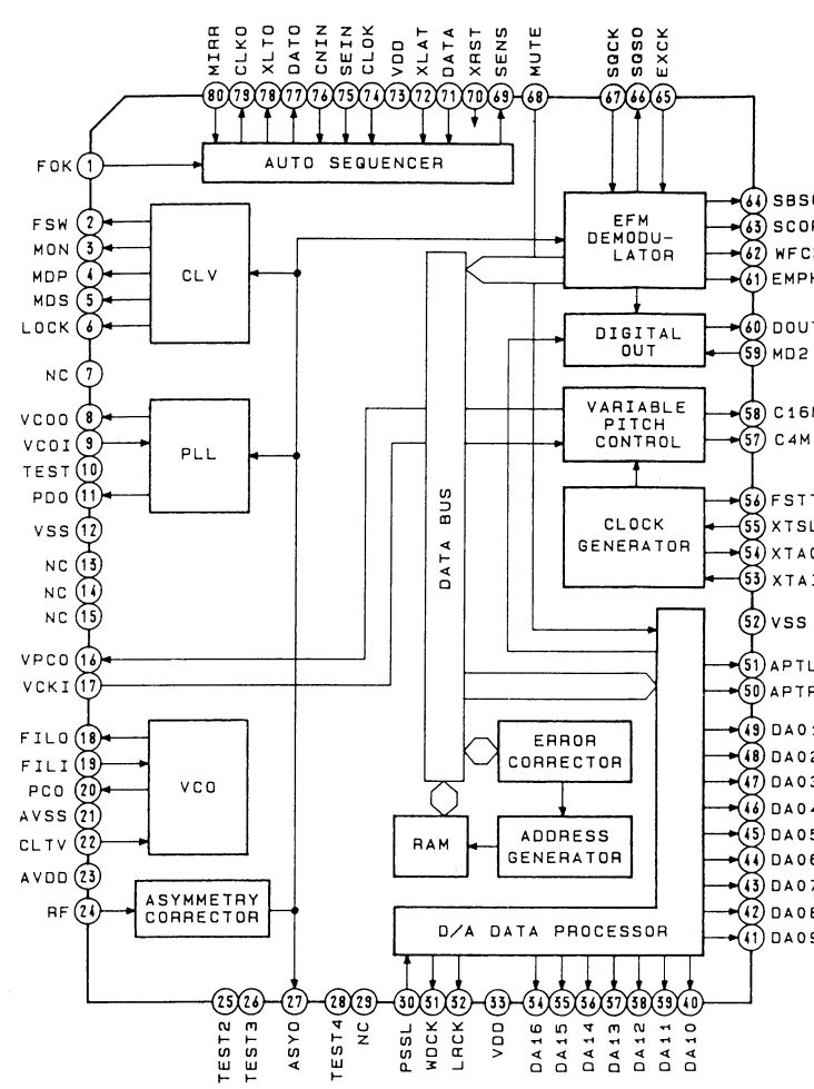
IC201 CXD2500AQ
