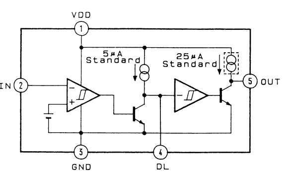
IC953 M51957AL
