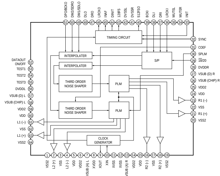
– AUDIO Section – IC302 CXD2562Q-CS
