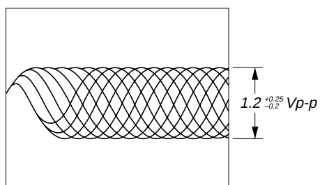
❶ IC107 ⑩ (RFO) 200 mV/DIV, 500 nsec/DIV
