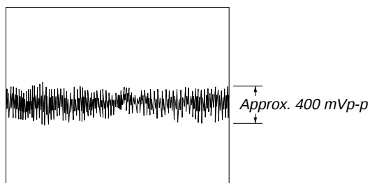
❷ IC107 ⑬ (TE) 200 mV/DIV, 100 μsec/DIV
