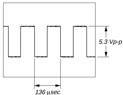
❻ IC105 ⑤⑤ (RFCK)
