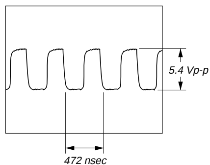
❺ IC105 ④⑦ (BCLK)
