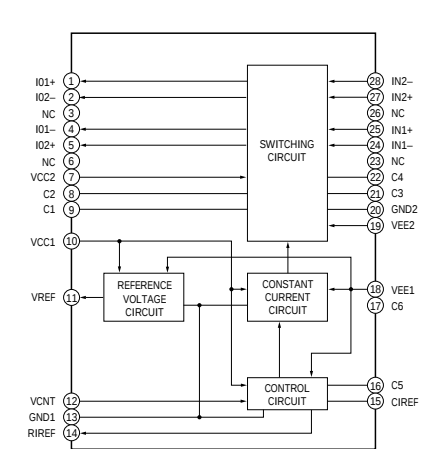
IC401, 501 CXA8042AS
