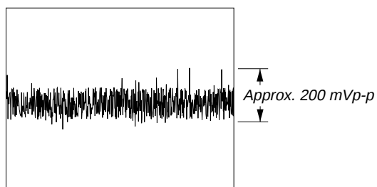
❸ IC107 ⑮ (FE) 200 mV/DIV, 50 nsec/DIV
