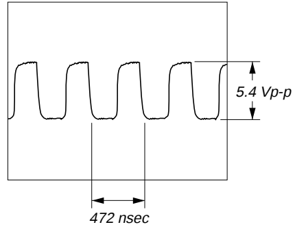
❺ IC105 ④⑦ (BCLK)
