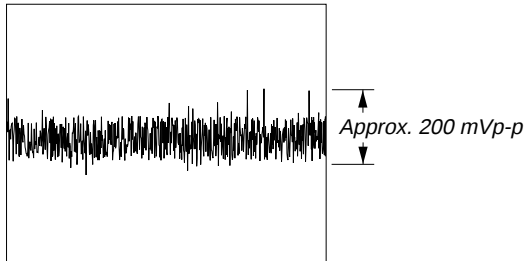
❸ IC107 ⑮ (FE) 200 mV/DIV, 50 nsec/DIV
