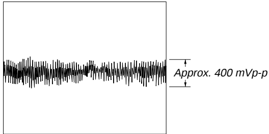
❷ IC107 ⑬ (TE) 200 mV/DIV, 100 μsec/DIV
