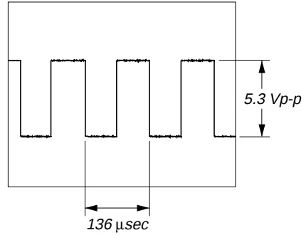
❻ IC105 ⑤⑤ (RFCK)
