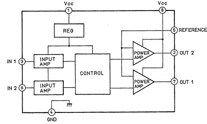
CXA1372Q
