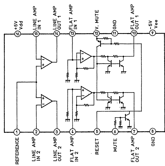
M54641L
