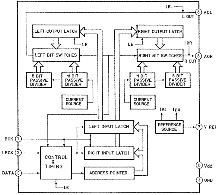
TDA1543
