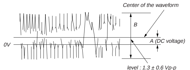
Traverse waveform
