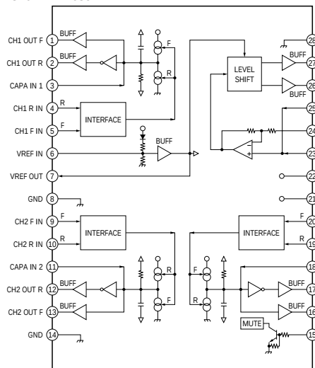
IC102 BA6392FP
