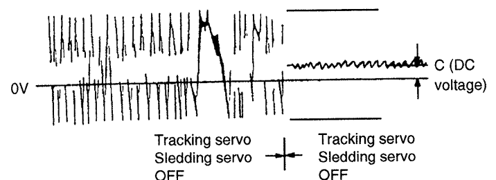
Traverse waveform
