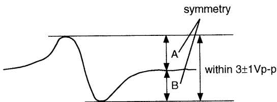
S-curve waveform
