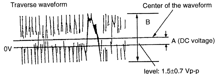
Traverse waveform
