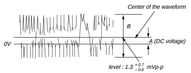
Traverse waveform
