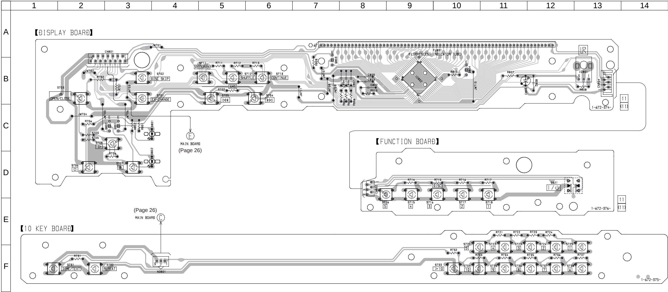
6-11. PRINTED WIRING BOARD DISPLAY SECTION • See page 17 for Circuit Boards Location.
