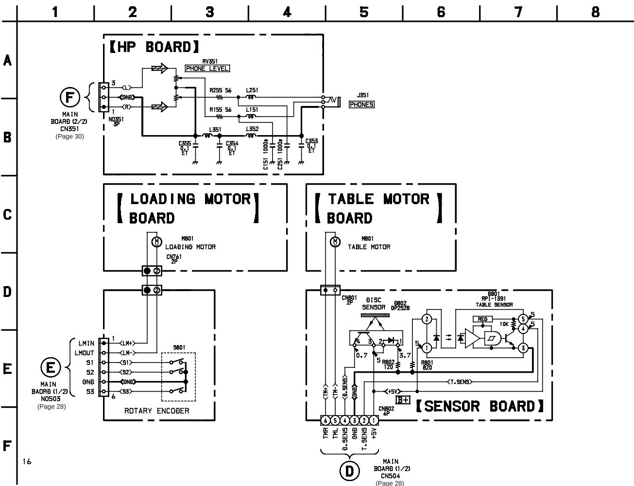
6-8. SCHEMATIC DIAGRAM HP SECTION
