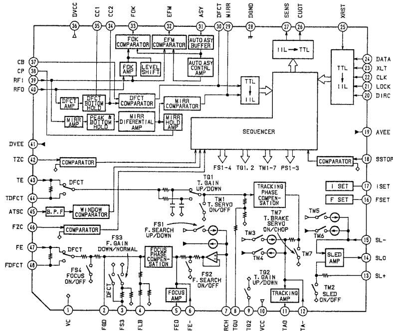
• IC101 CXD1372Q
