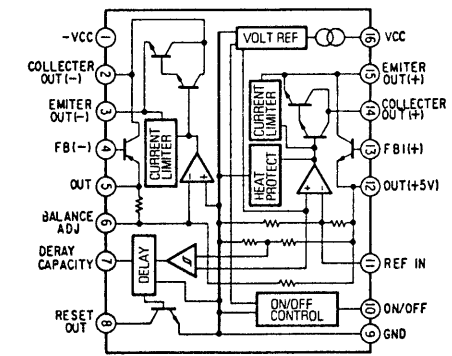
• IC351 CXD2554P
