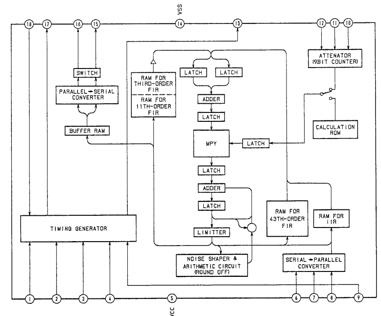
• IC351 CXD2554P
