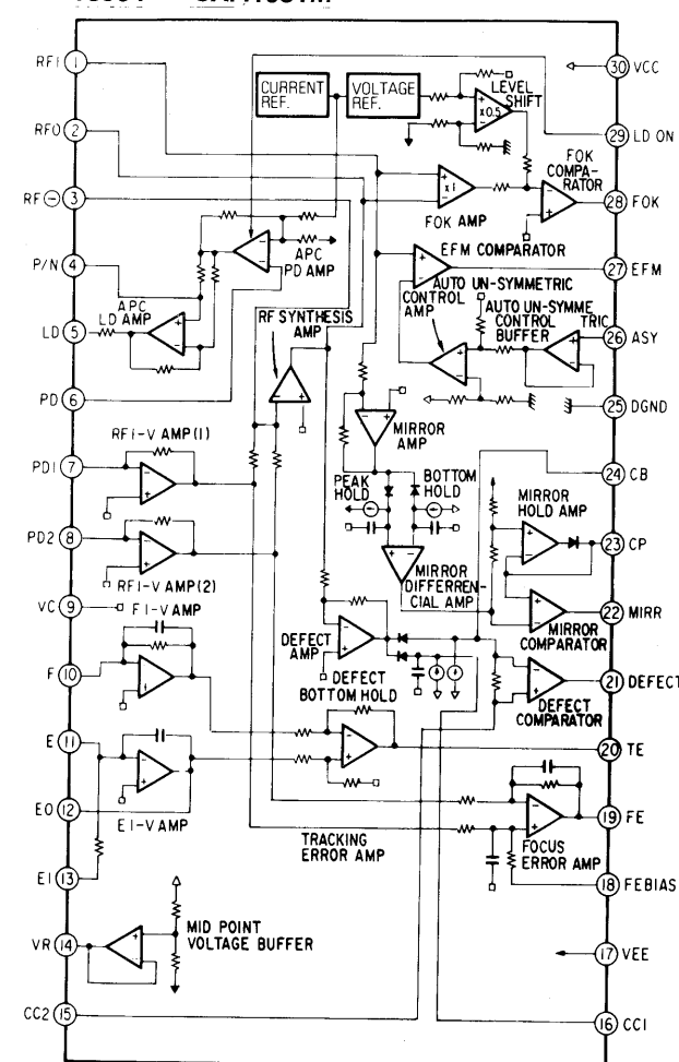
IC504 CXA1081M
