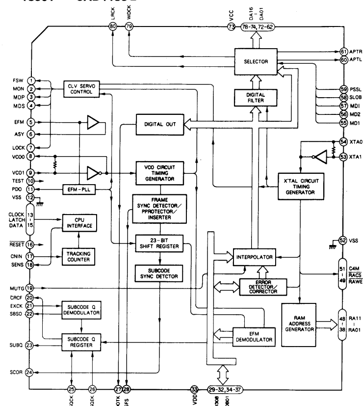
IC501 CXD1135Q
