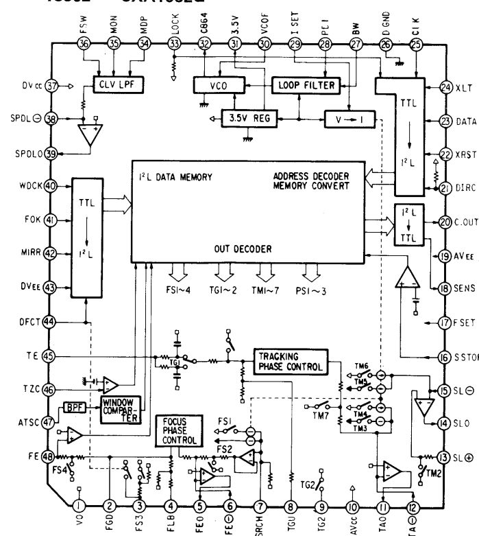
IC502 CXA1082Q
