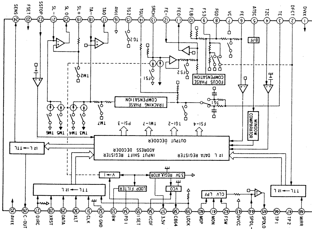
IC201 CXA1082BS
