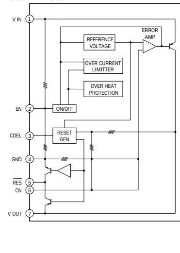
IC601 LA5602
