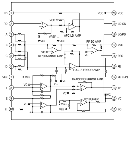
IC103 CXA1821M
