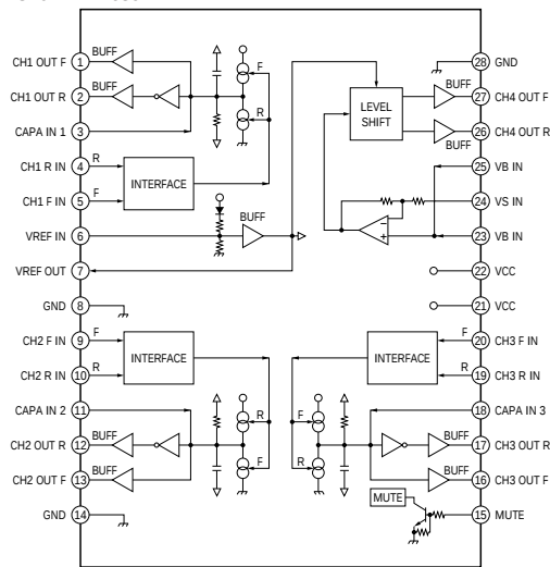
IC102 BA6392FP
