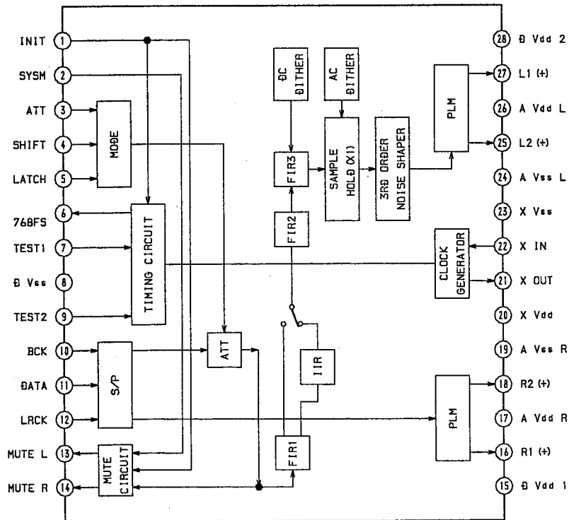
IC103 CXD2565M
