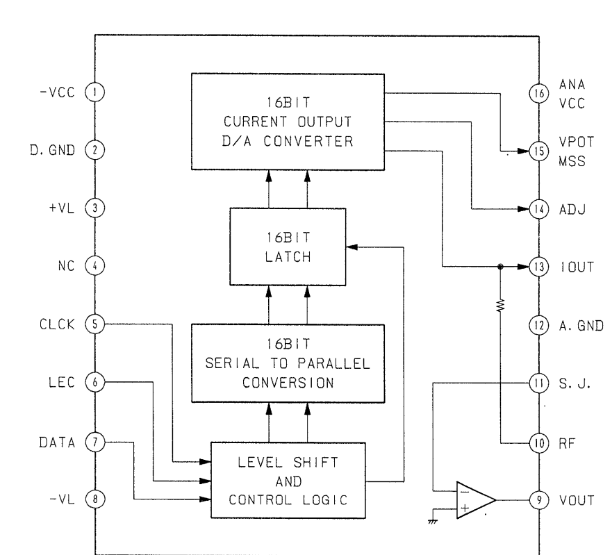
IC501, 601 PCM56P
