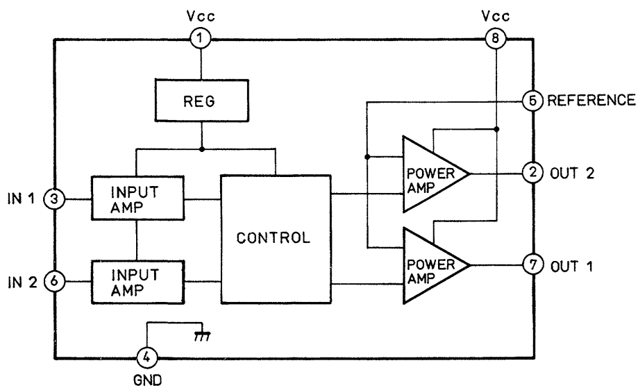
IC103 M54641L
