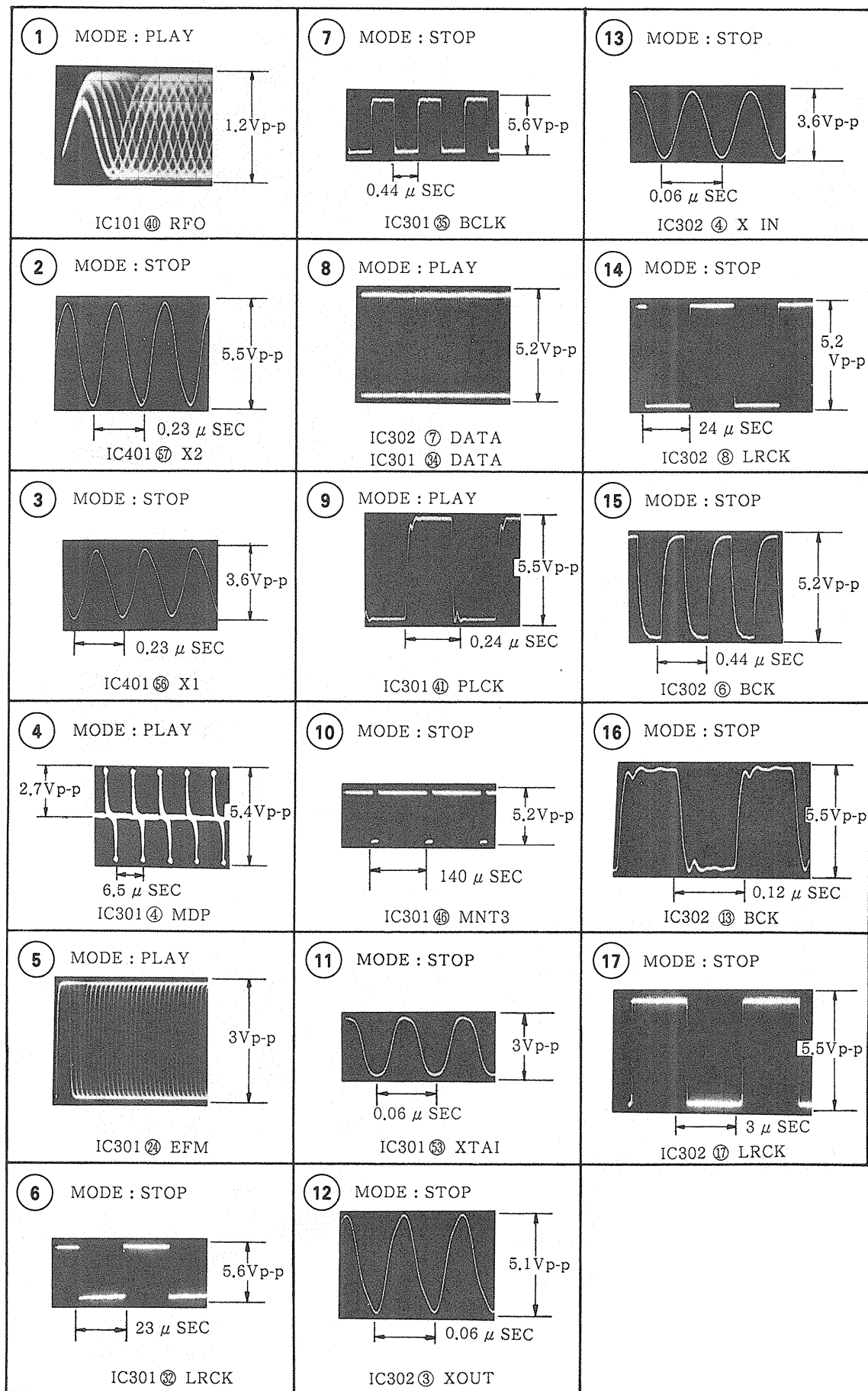
5-1. WAVEFORMS
