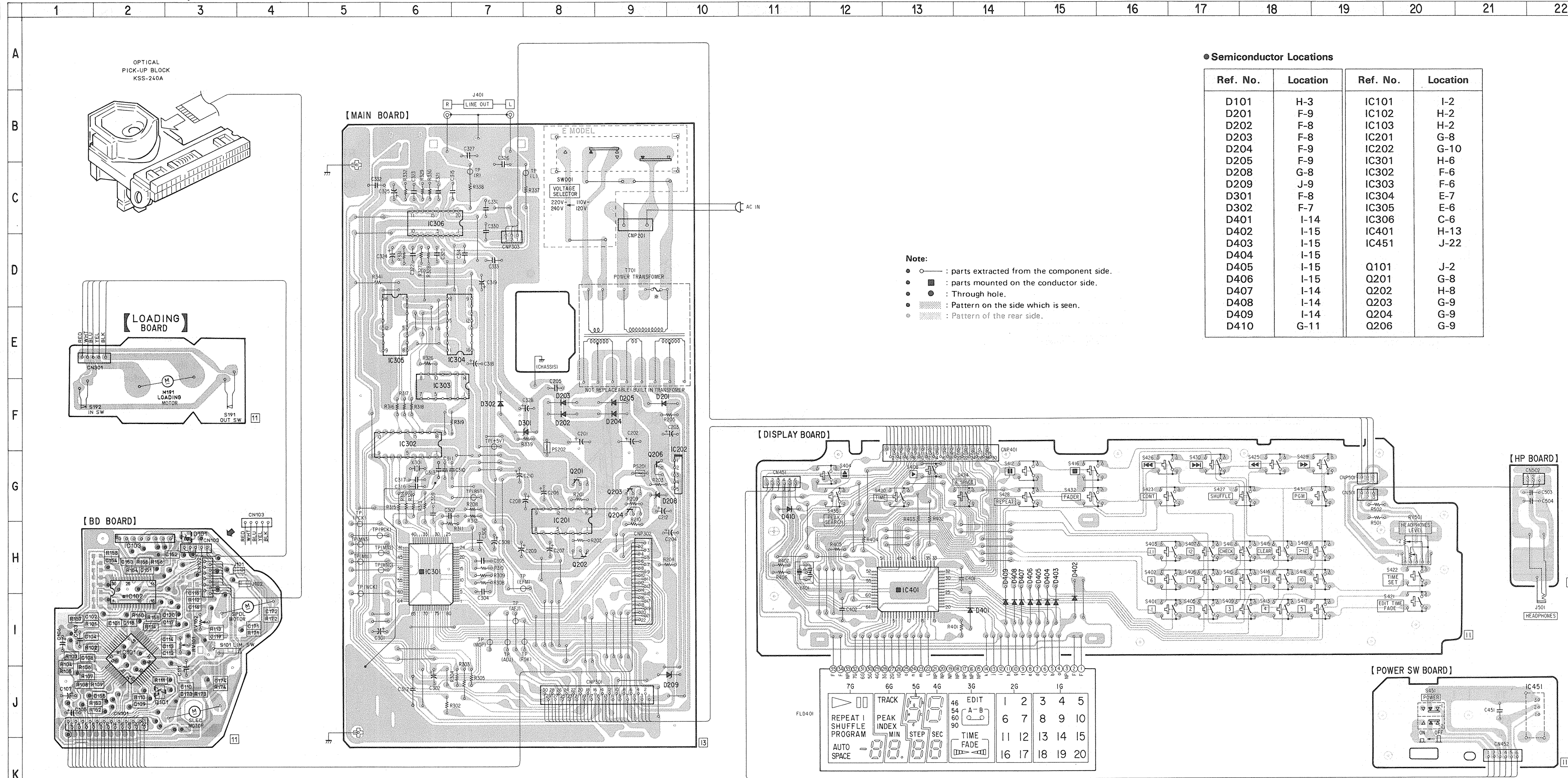
5-2. PRINTED WIRING BOARDS
