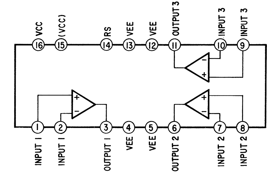
IC202, 203 LA6520
