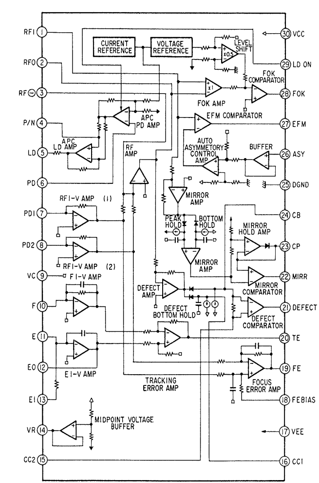
IC101 CXA1081S
