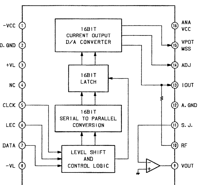
IC304, 305 PCM56
