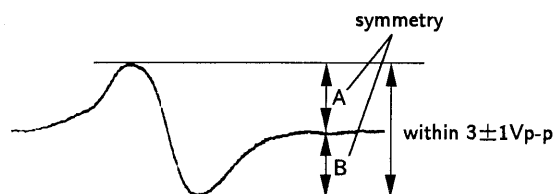
S-curve waveform
