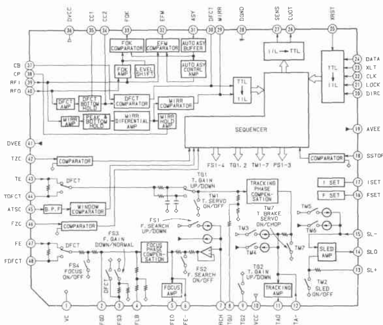
IC101 CXA1372Q
