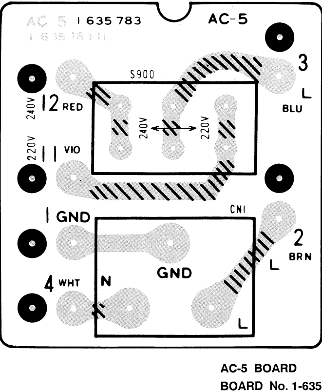
AC-5 BOARD (EK MODEL)
