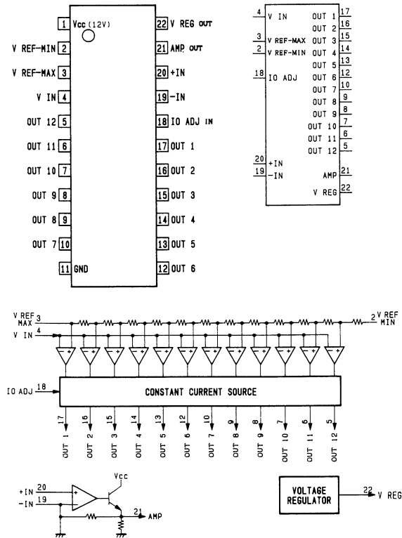
IR2E30 (SHARP) 12-DOT LED DISPLAY DRIVER - TOP VIEW -
