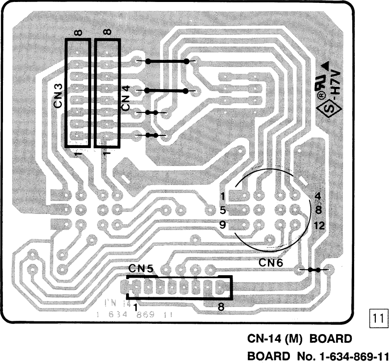
CN-14 (M) BOARD
