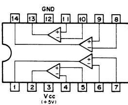
LM339N (TI) QUAD COMPARATORS - TOP VIEW -
