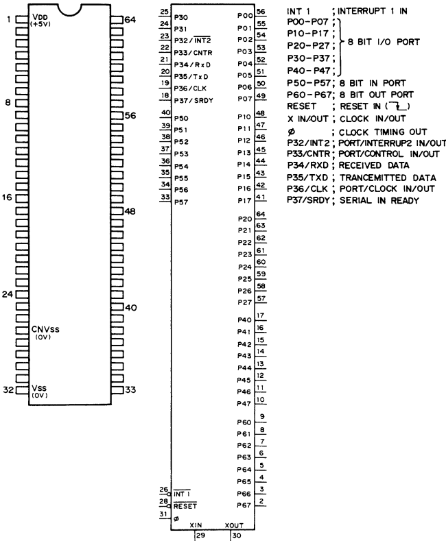
M5074SP-C42SP (FUJITSU) C-MOS PROCESS 8-BIT ONE CHIP MICROCOMPUTER - TOP VIEW -
