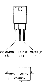
NJM7912FA (JRC) - 12V NEGATIVE VOLTAGE REGULATOR (500mA) - FRONT VIEW -
