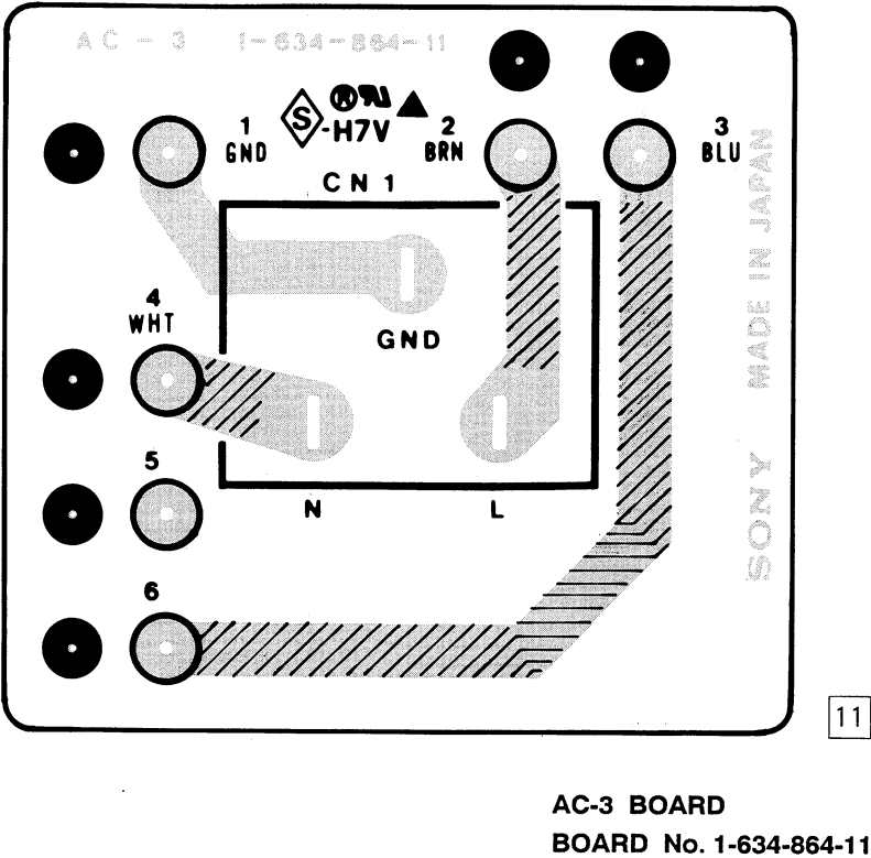
AC-3 BOARD (J, U MODEL)
