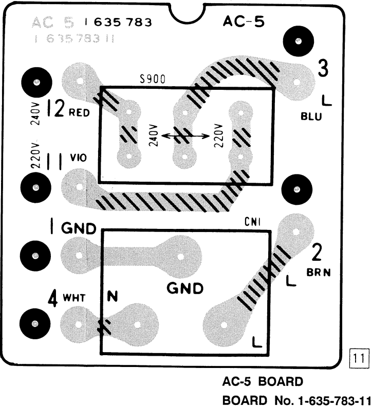
AC-5 BOARD (EK MODEL)
