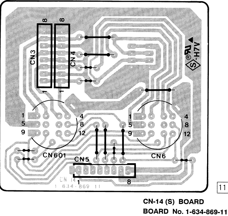
CN-14 (S) BOARD
