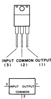
NJM7805FA (JRC) + 5V POSITIVE VOLTAGE REGULATOR (500mA) - FRONT VIEW -
