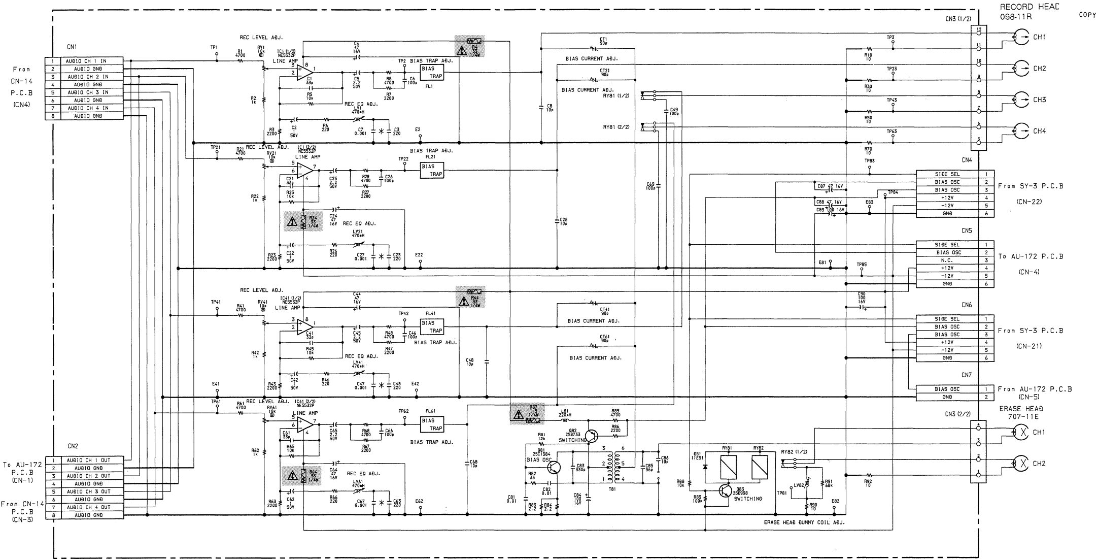
AU-171 BOARD BOARD No. 1-643-616-11
