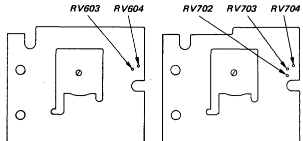
SERVO BOARD (A) (DECK A side)
