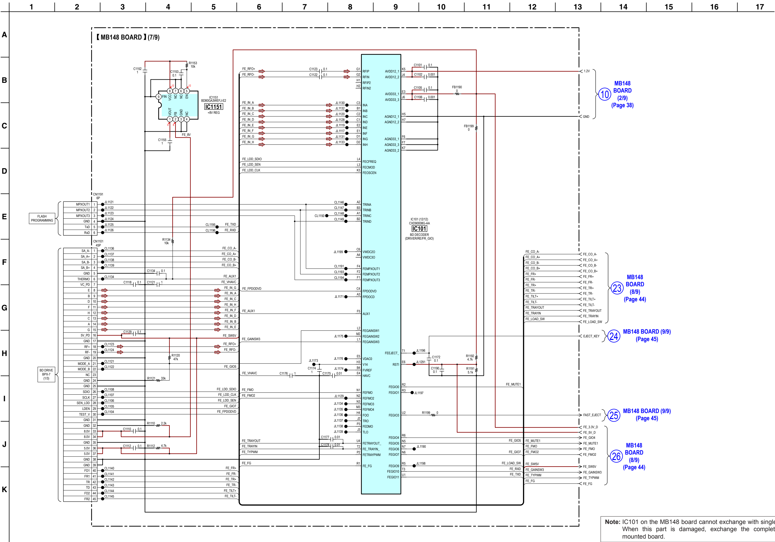
5-14. SCHEMATIC DIAGRAM - MB148 Board (7/9) - • See page 61 for IC Pin Function Descriptions.
