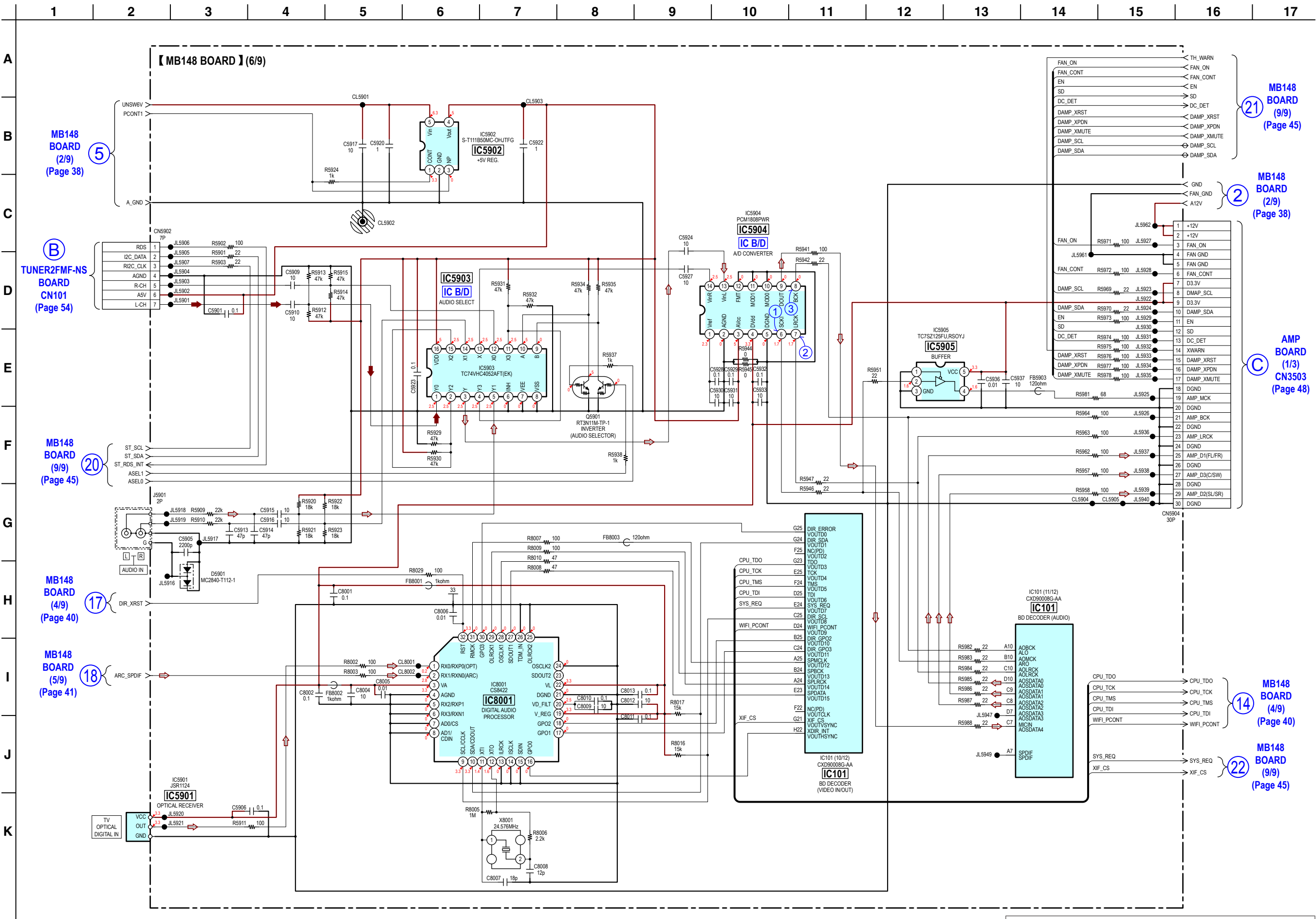
5-13. SCHEMATIC DIAGRAM - MB148 Board (6/9) - • See page 53 for Waveforms. • See page 55 for IC Block Diagrams. • See page 61 for IC Pin Function Descriptions.
