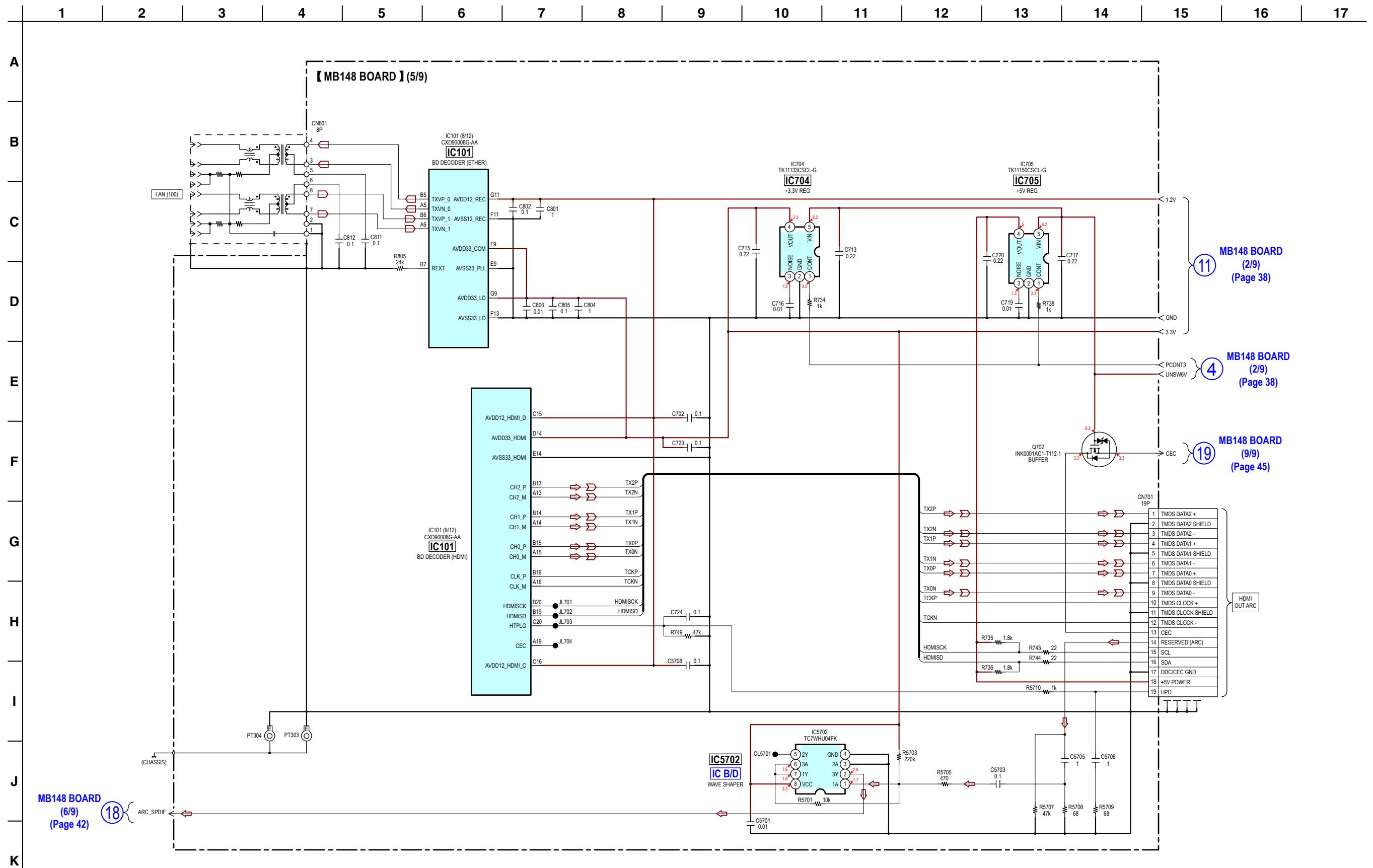
5-12. SCHEMATIC DIAGRAM - MB148 Board (5/9) - • See page 55 for IC Block Diagrams. • See page 61 for IC Pin Function Descriptions.
