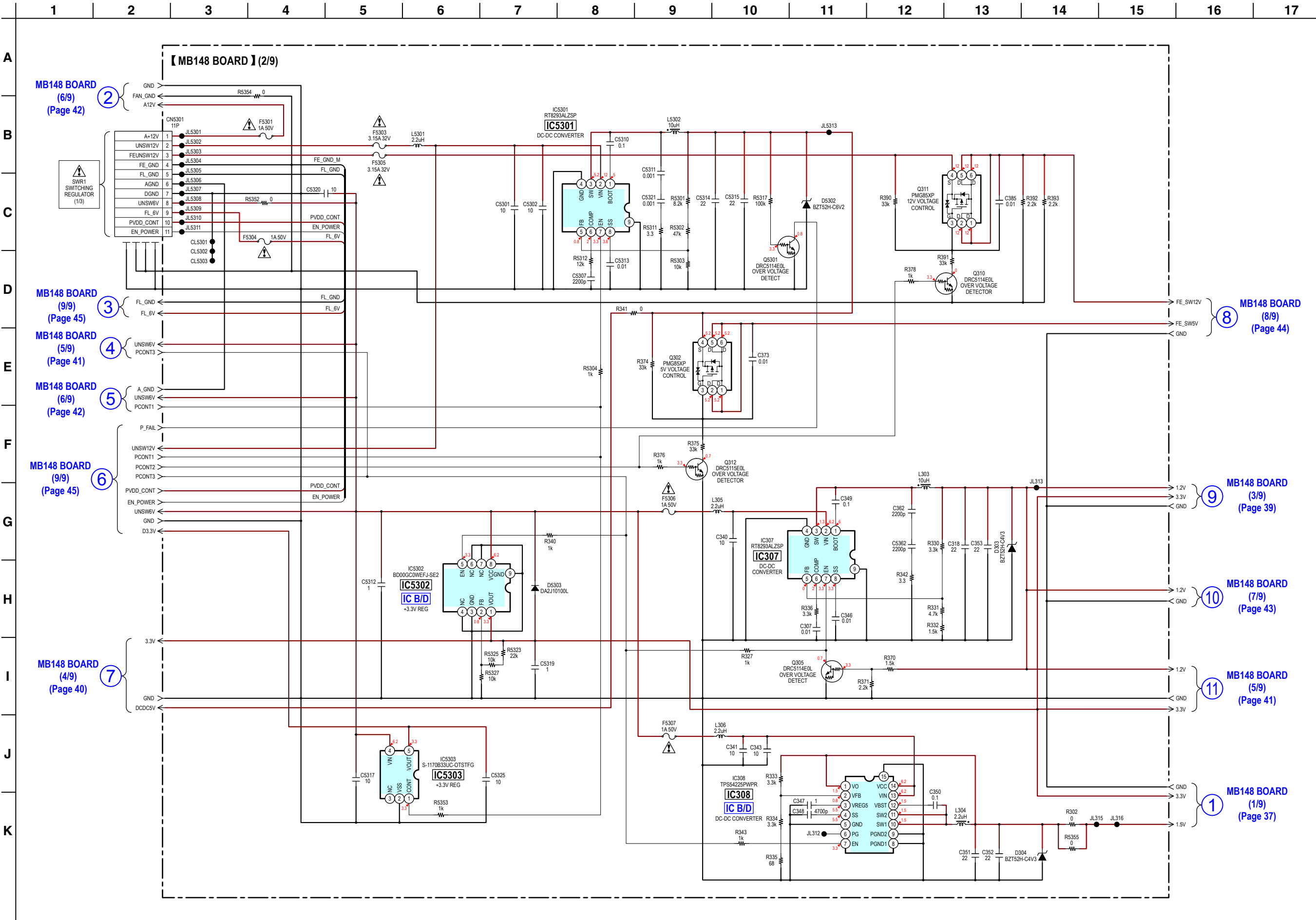
5-9. SCHEMATIC DIAGRAM - MB148 Board (2/9) - • See page 55 for IC Block Diagrams.
