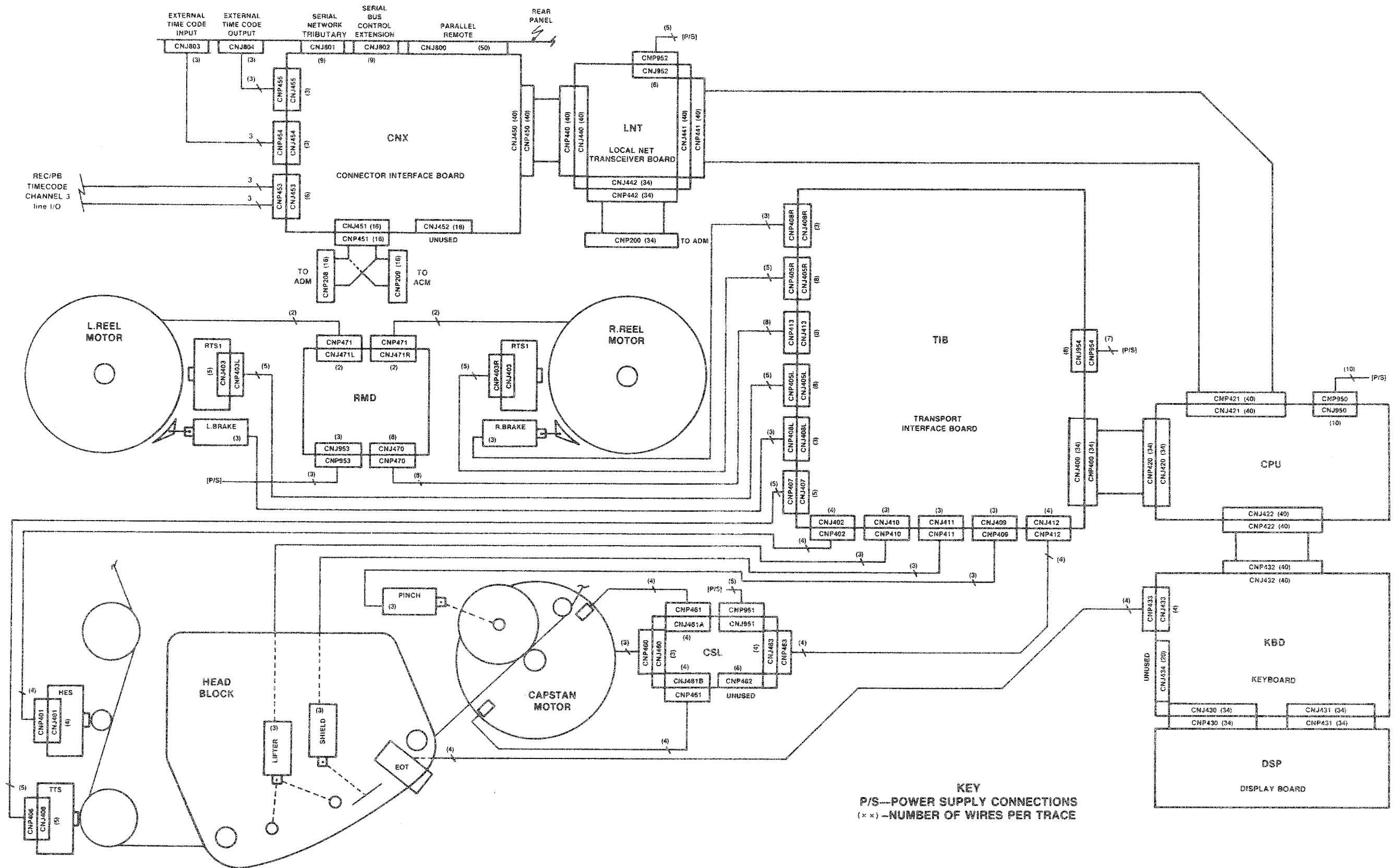
TAPE TRANSPORT BLOCK DIAGRAM
