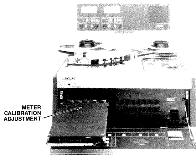
Figure 3-4. CNL Adjustments
