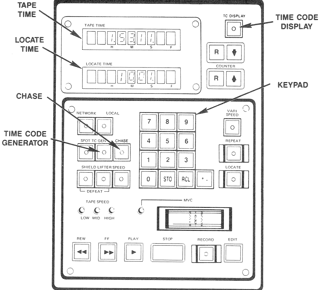
Figure 2-1. Transport Control Panel
