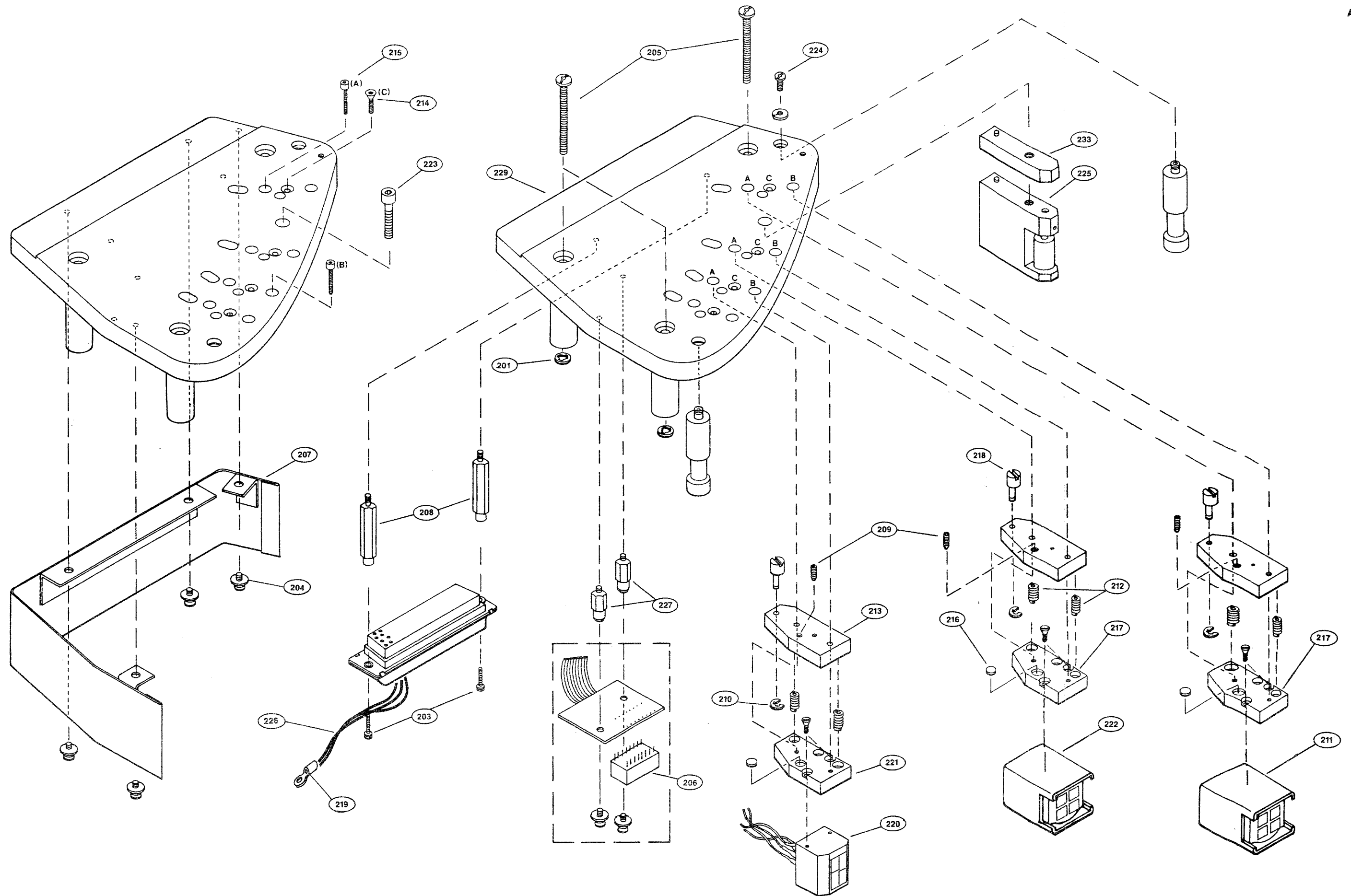
Figure 3-2. 1/2" 2-Track Headstack
