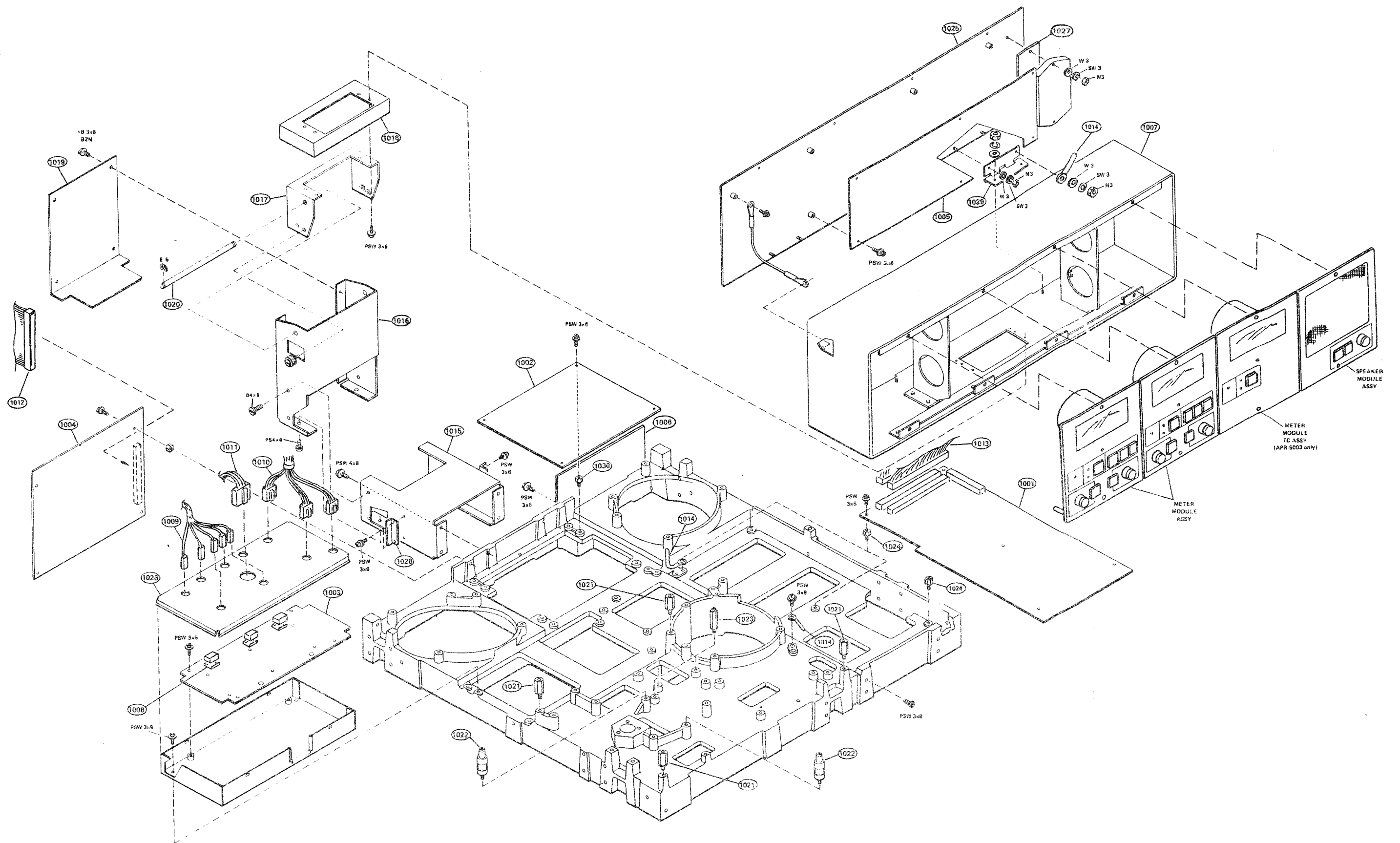
Figure 5-2. Chassis Assembly
