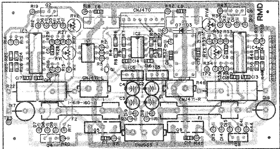
SOLDER SIDE PATTERN 1-619-160-11 COMPONENT SIDE PATTERN 1-619-160-11
