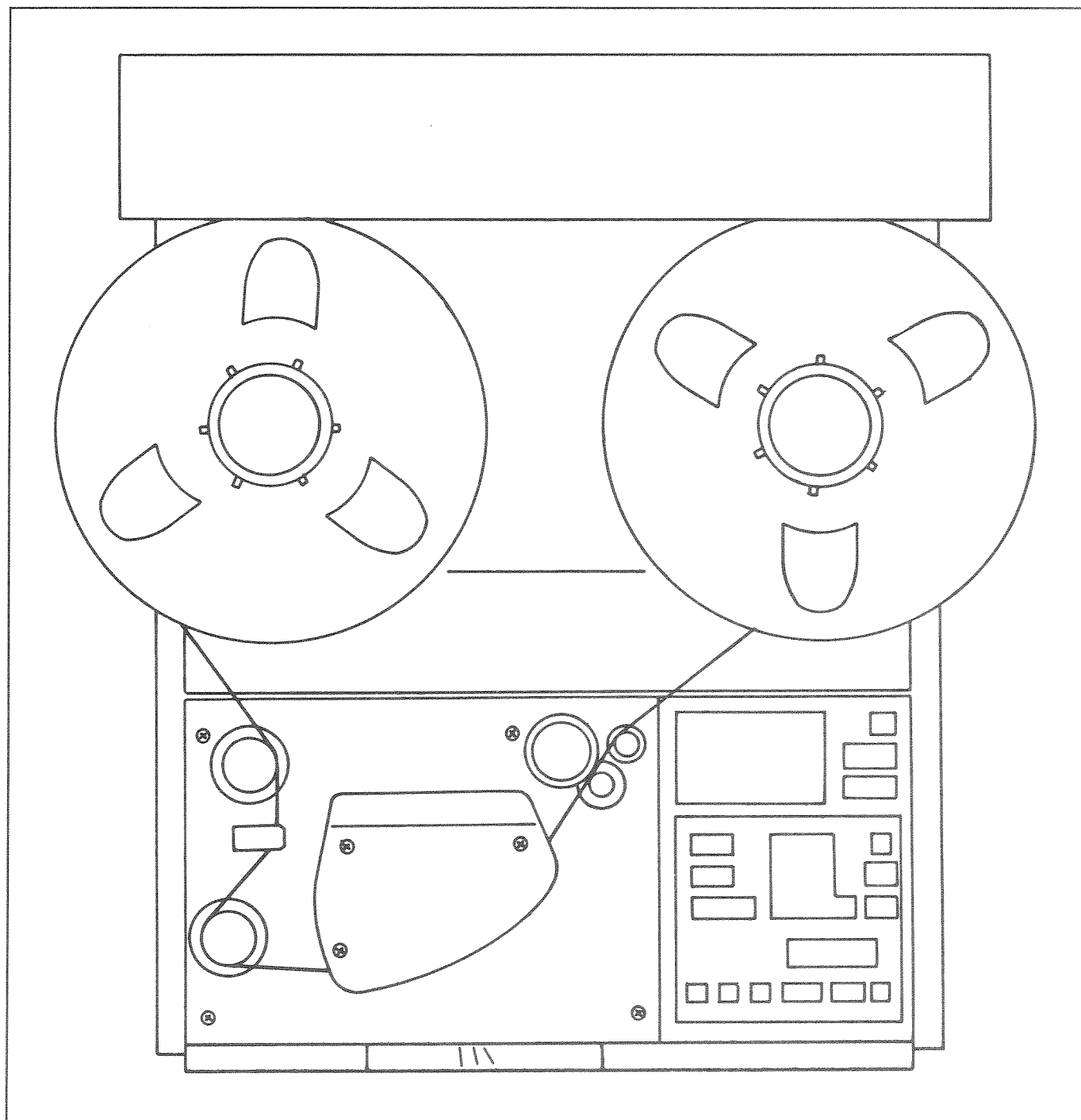
Figure 2-2. Tape Path
