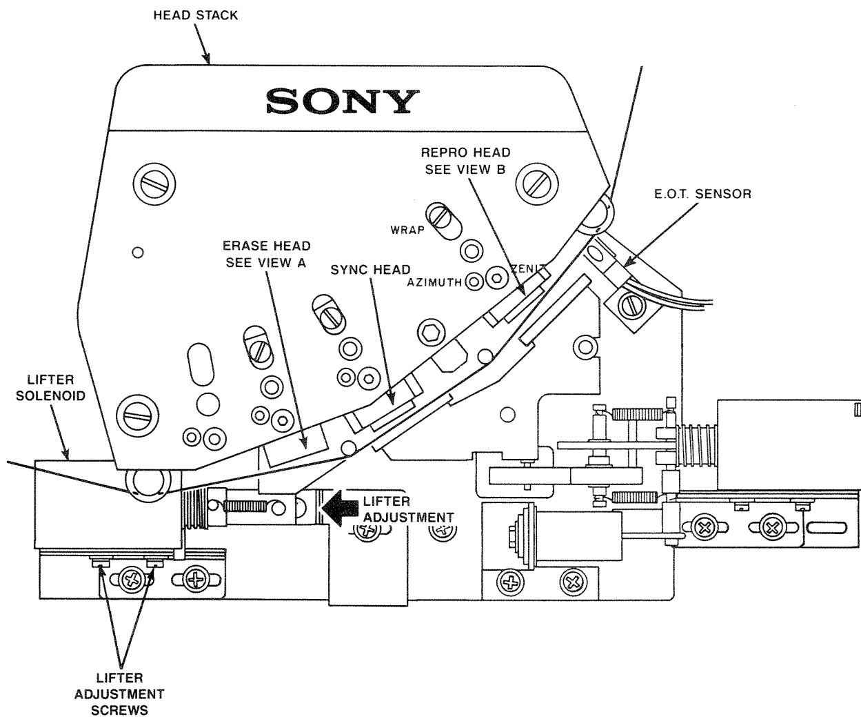
Figure 6-29. Lifter Adjustment
