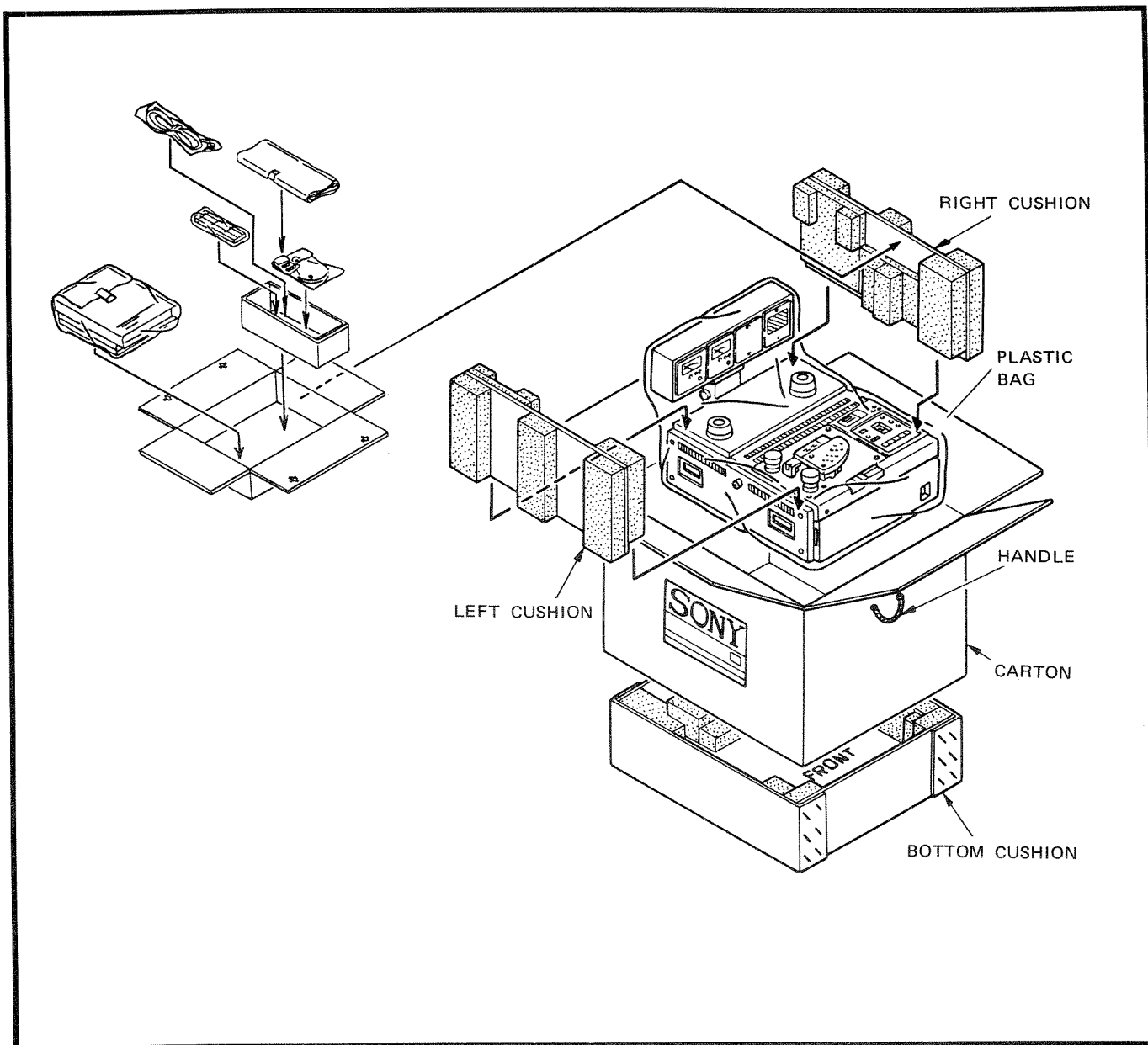
Figure 2-1. APR-5000 Packaging
