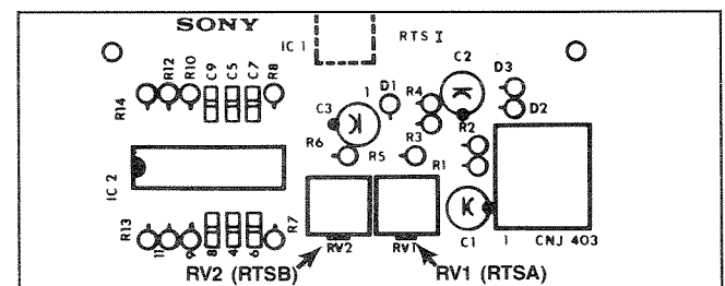
Figure 6-17. RTS PC Board
