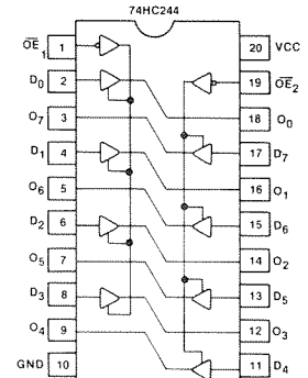
OCTAL BUFFER/LINE DRIVER 74HC244 FUNCTION TABLE
