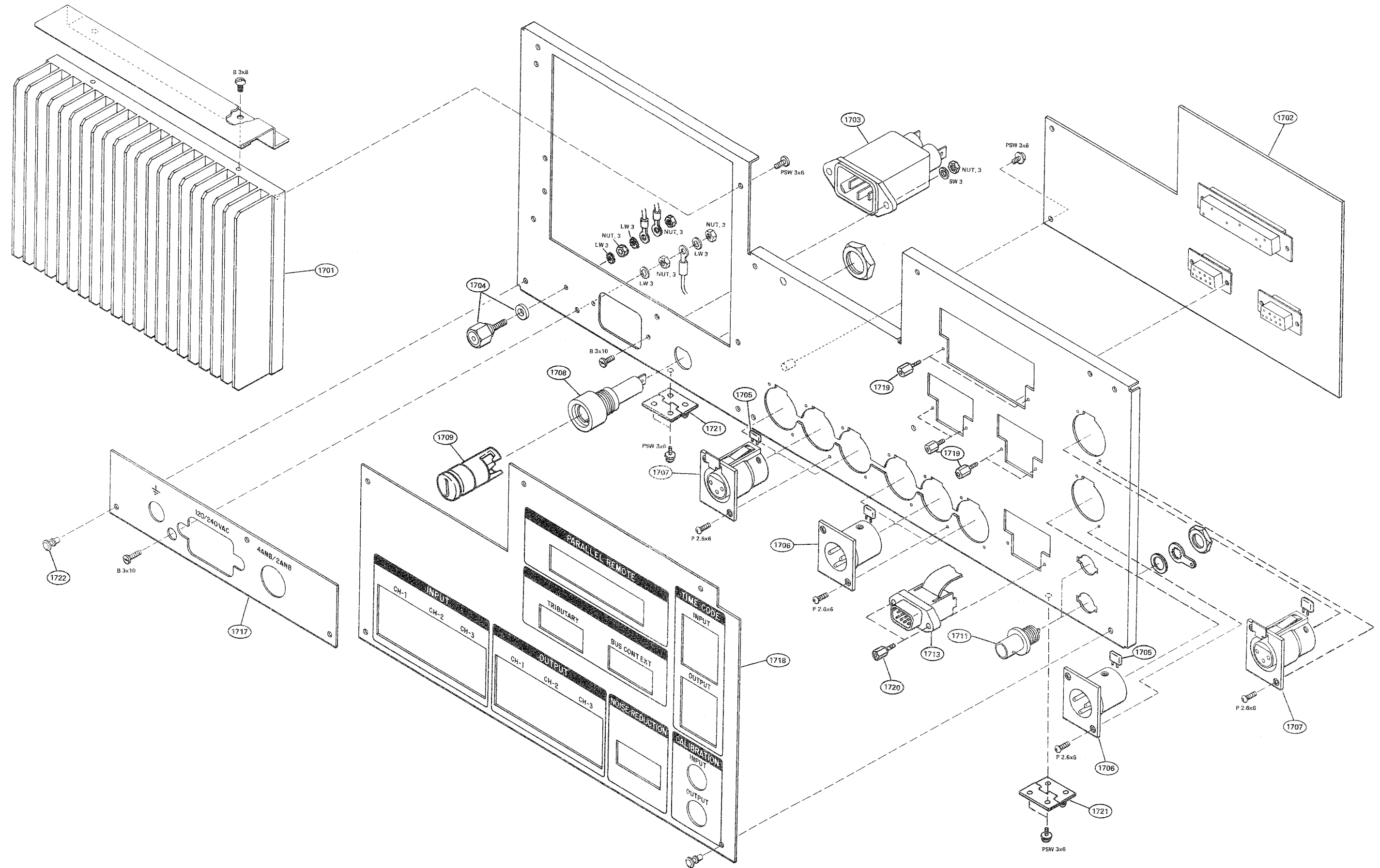
REAR PANEL ASSY (For APR-5002)
