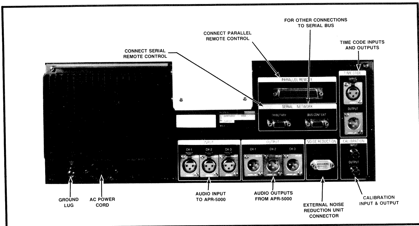
Figure 3-2. Connector Diagram
