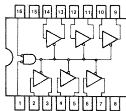
HEX BUFFER WITH ENABLES
