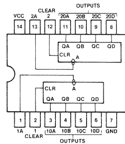
DUAL 4-BIT BINARY COUNTER
