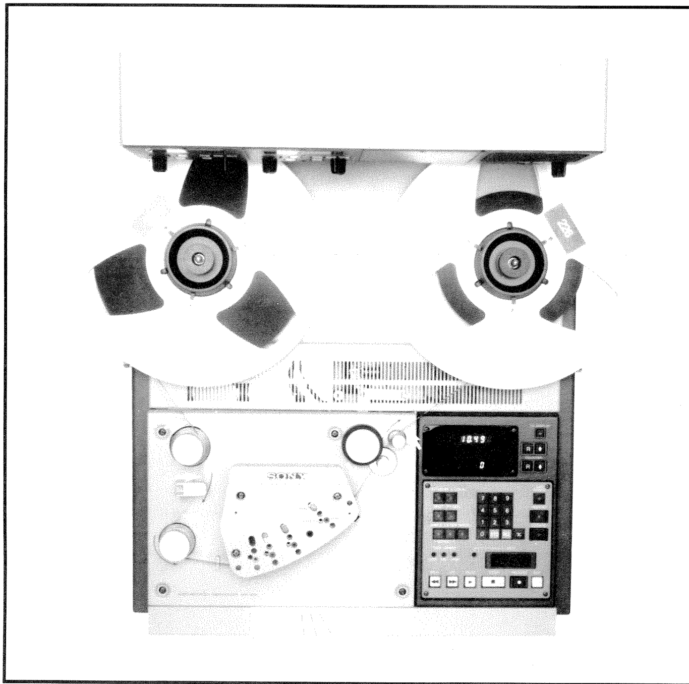
Figure 5-2. Threading Tape
