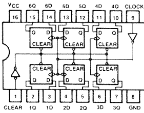
HEX D-TYPE FLIP-FLOPS 74HC174
