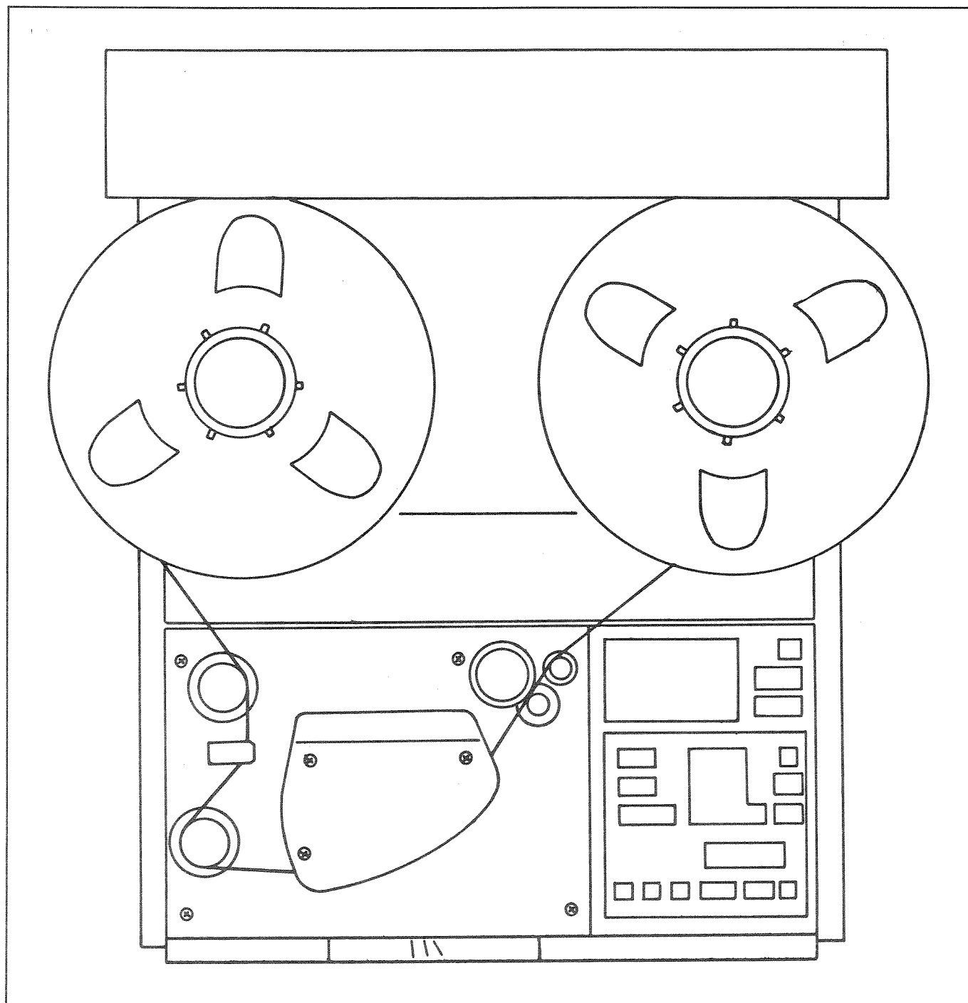
Figure 4-10. Tape Path
