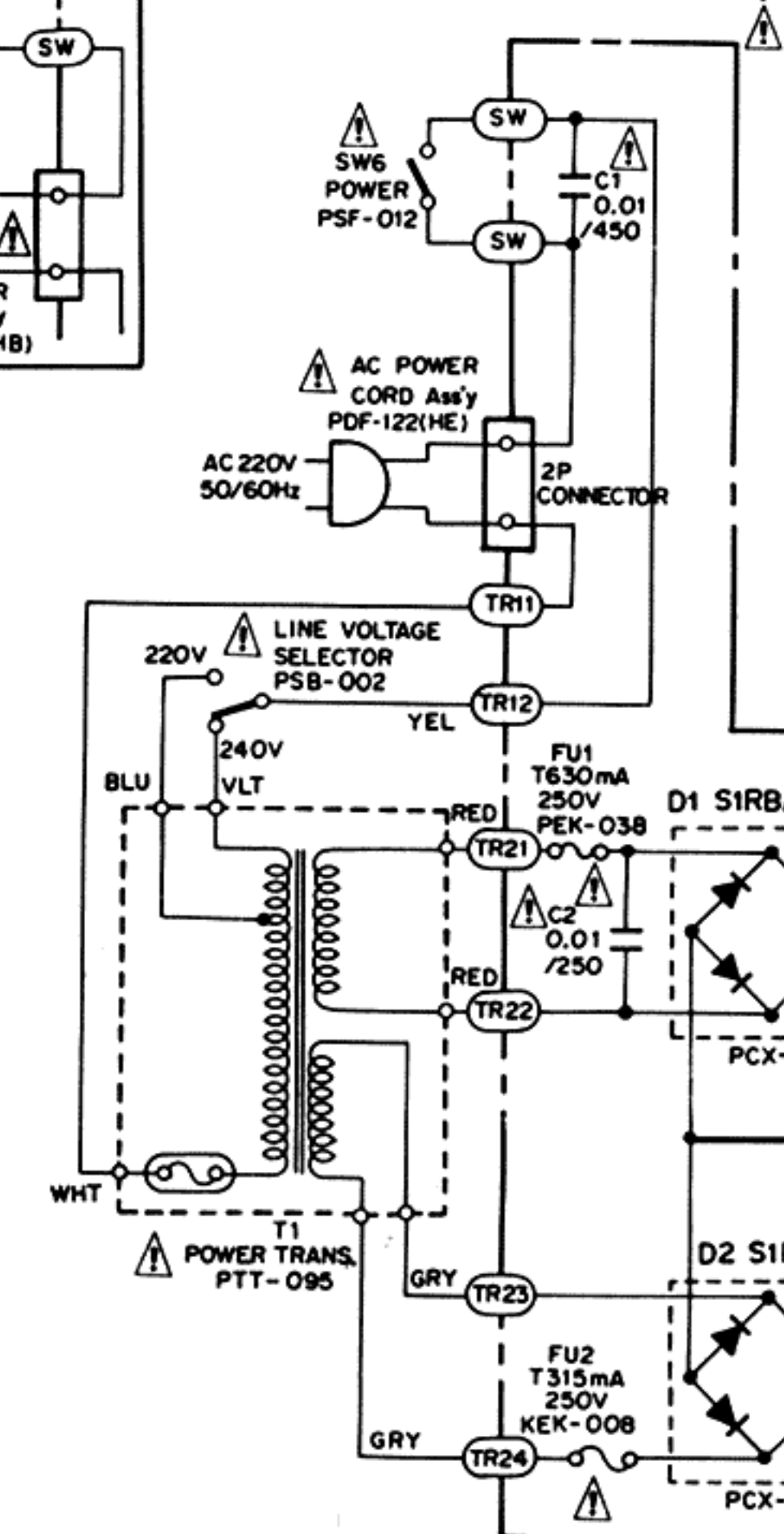
POWER SUPPLY Assy
