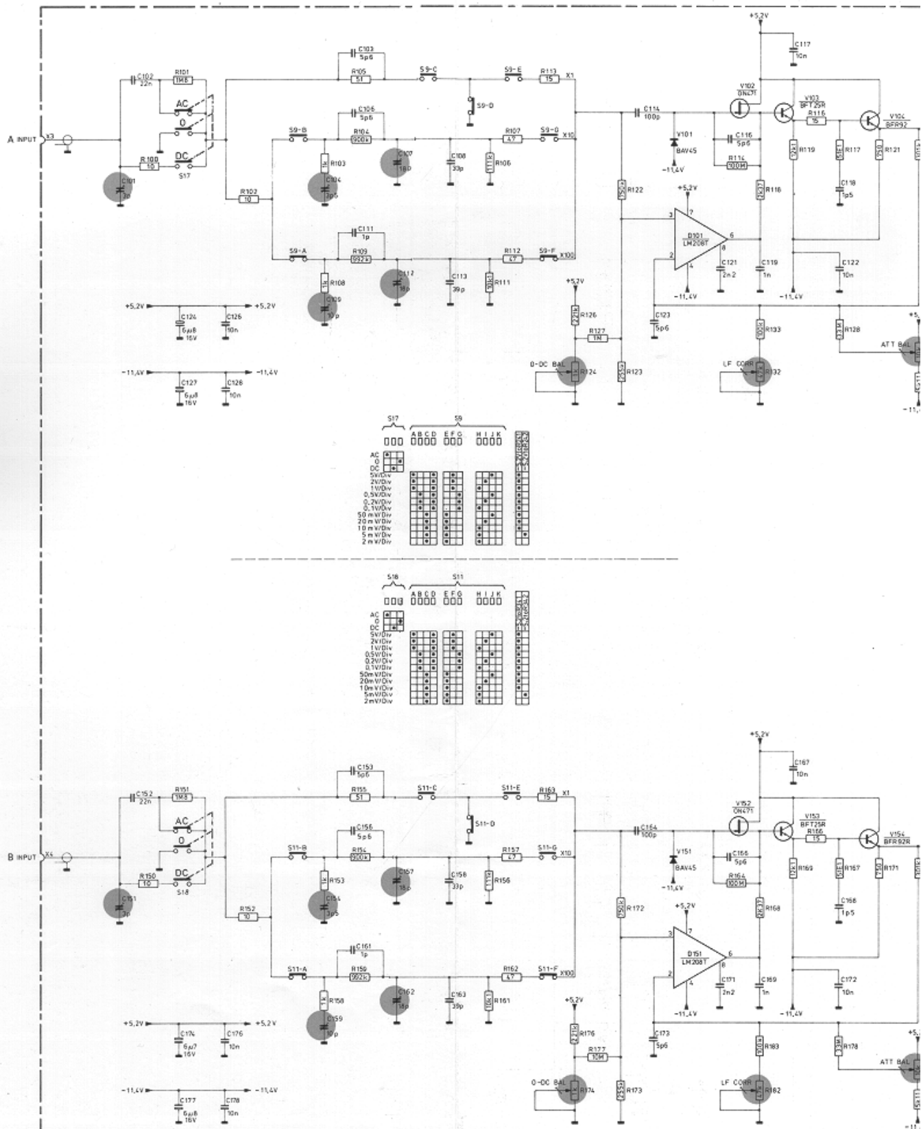
UNIT 2 CH.A AND CH.B ATTENUATOR
