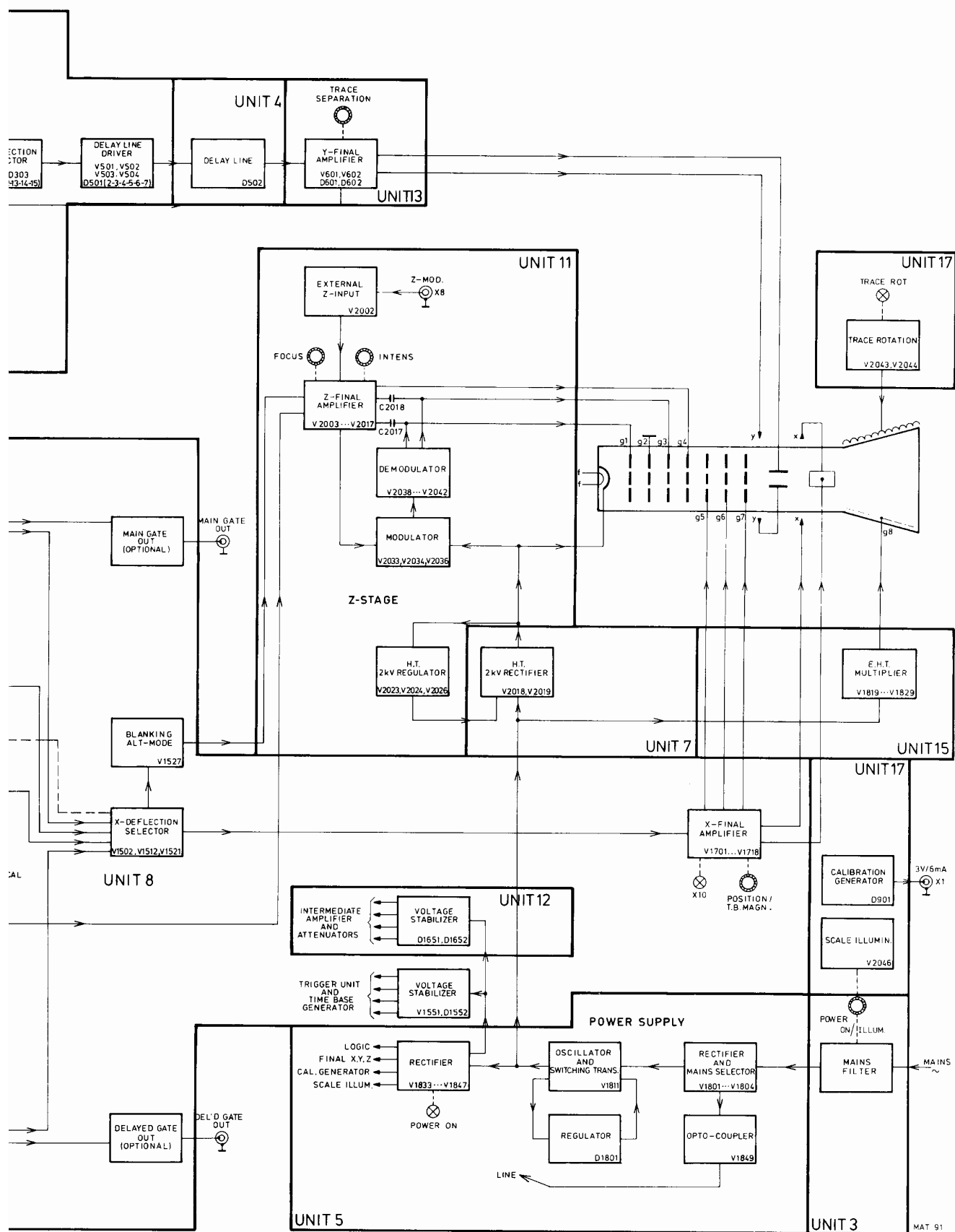
Fig. 3.1. Block diagram
