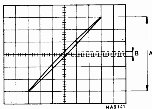
Fig. 3.23. Phase difference in X-Y mode
