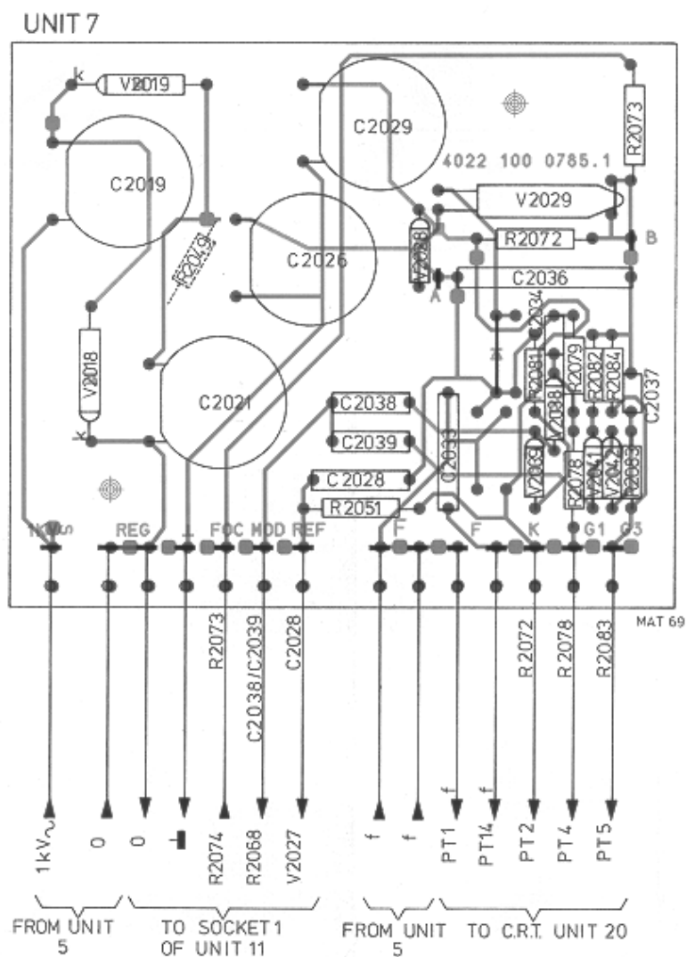
Fig. 3.43. Focus unit (UNIT 7)
