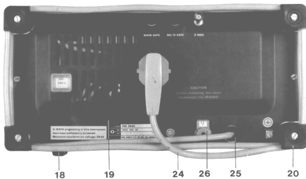
Fig. 3.38. Rear view showing itemnumbers
