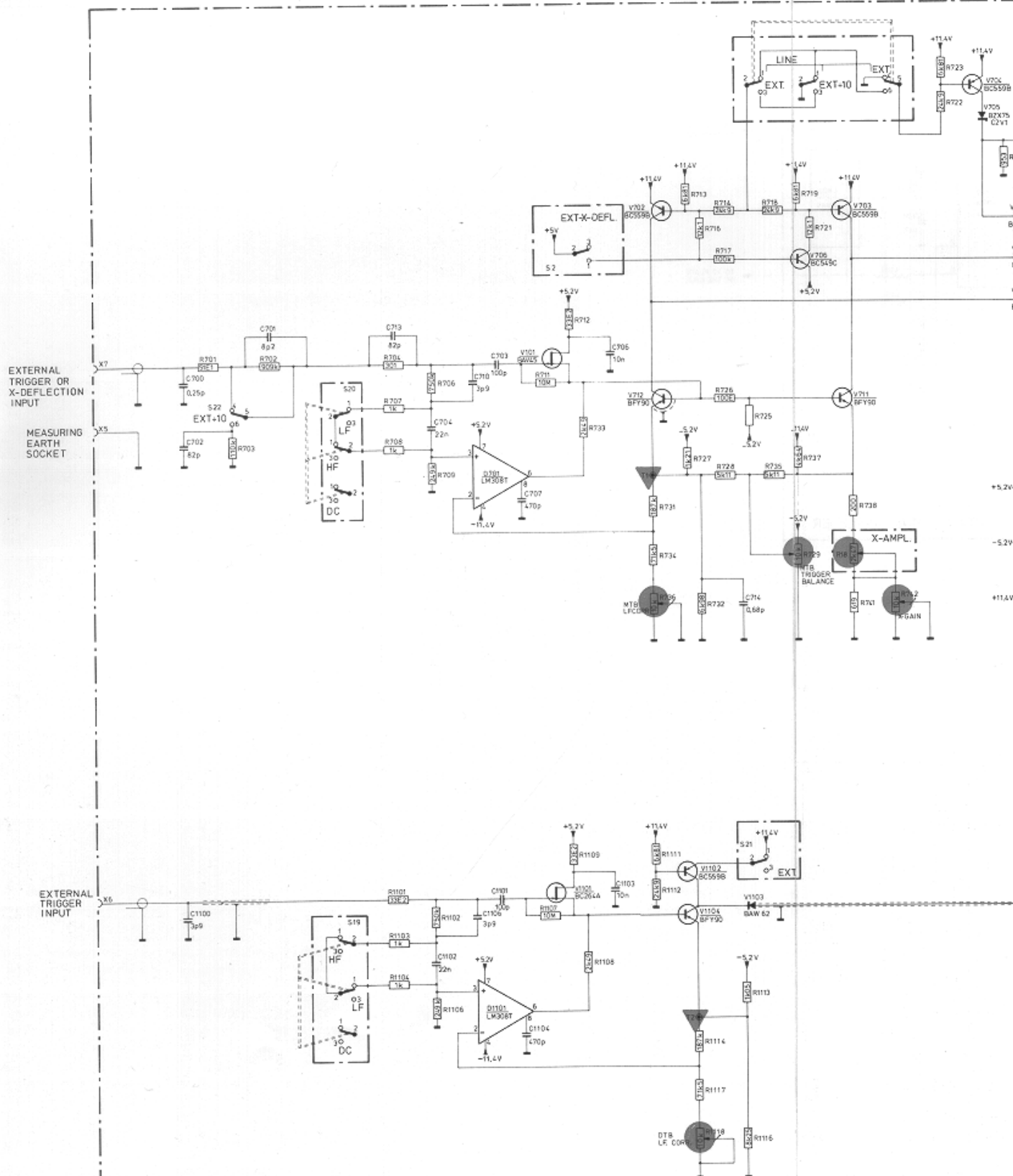
UNIT 16 MTB AND DTB EXTERNAL INPUT UNIT
