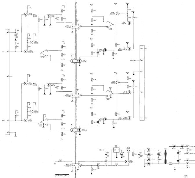
Fig. 7.15. Galvanic separation
