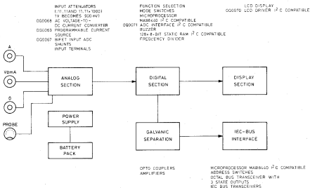
Fig. 2.1. Basic built-up of PM 2519
