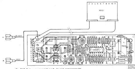
Fig. 7.13. Battery power supply p.c.b., lay-out, component side
