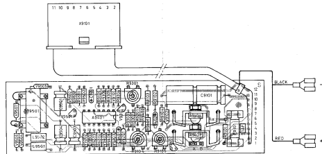
Fig. 7.14. Battery power supply p.c.b., lay-out, conductor side
