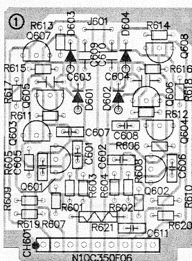
PRE MODULE BOARD
