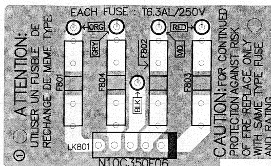
FUSE BOARD
