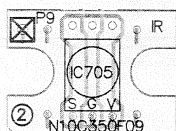
IR RECEIVER BOARD
