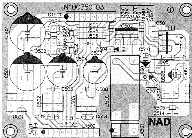
STANDBY BOARD
