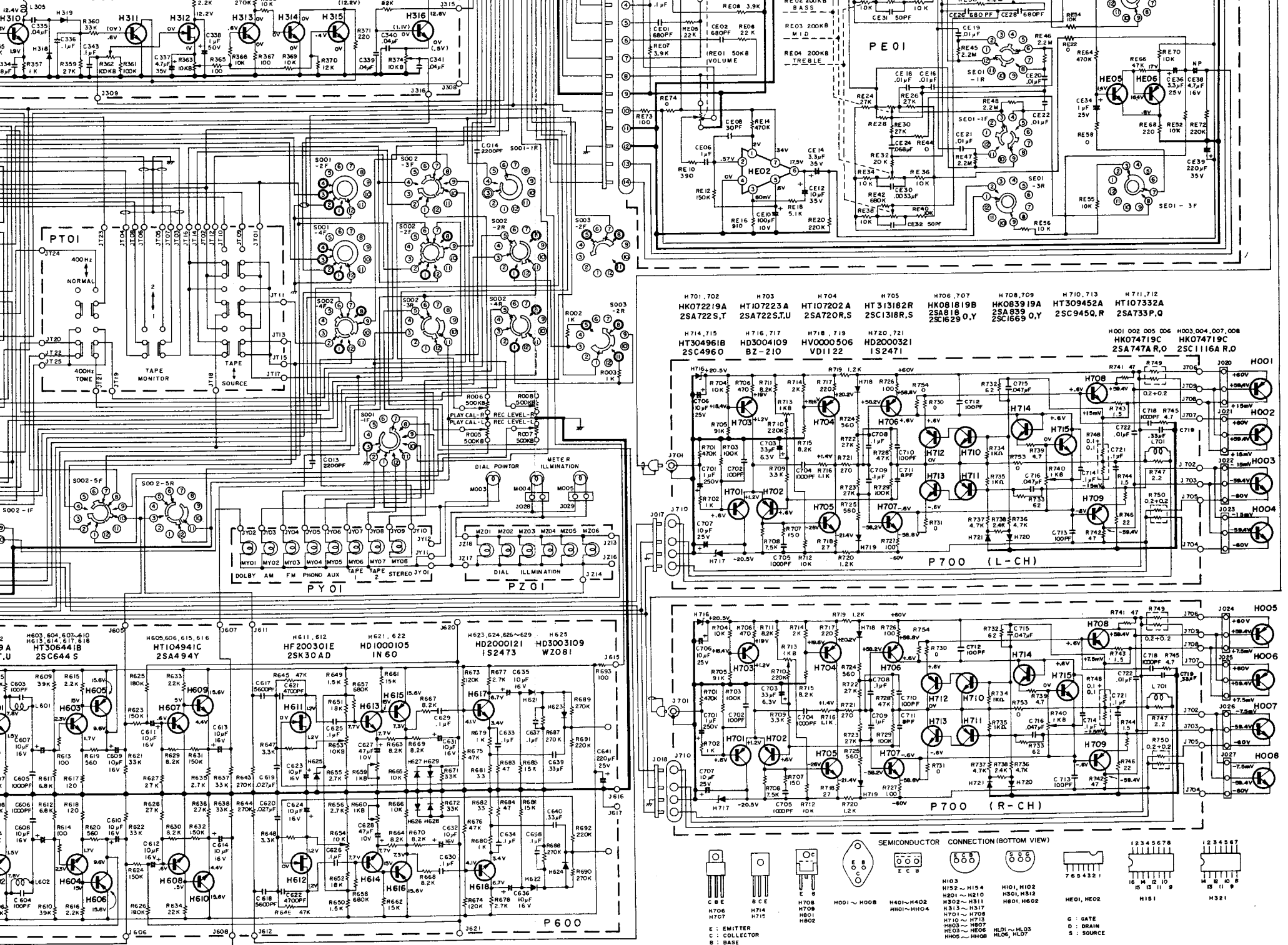
Figure 30. Schematic Diagram
