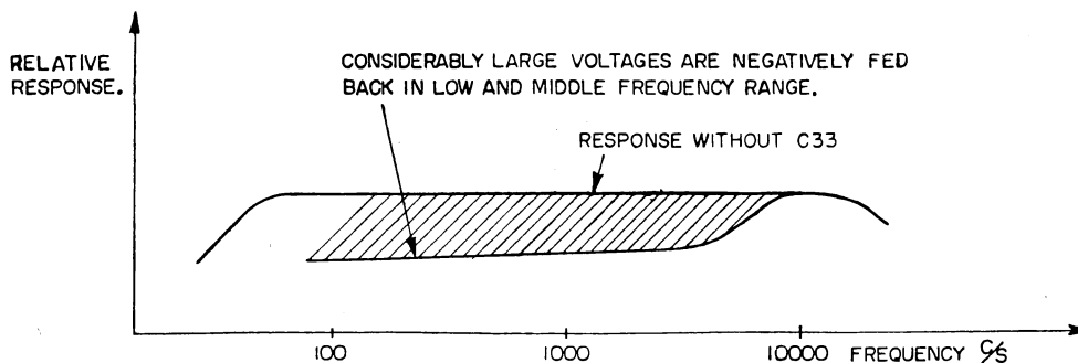
Fig. 3 HIGH FREQUENCY BOOSTING.
