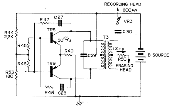
Fig. 12 BIAS OSCILLATION CIRCUIT.
