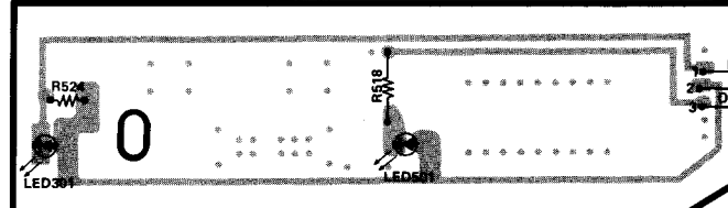
LED P.W.B.
