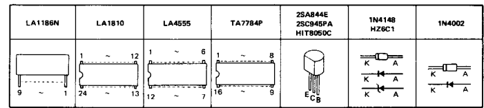
GRAPHIC EQUALIZER CONTROL
