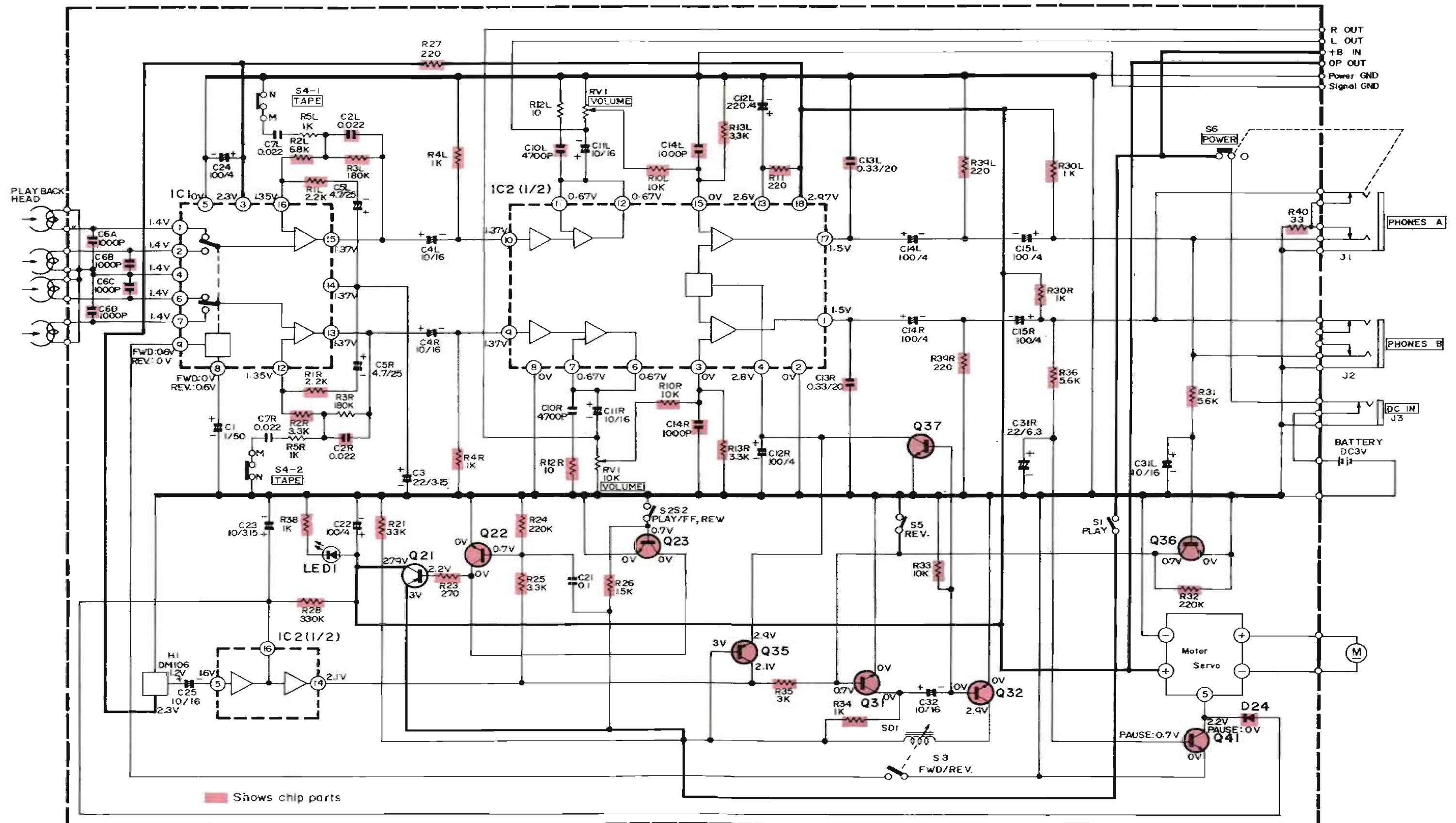
SCHEMATIC DIAGRAM [Stereo Cassette Player (TAPE 1 ) Section]
