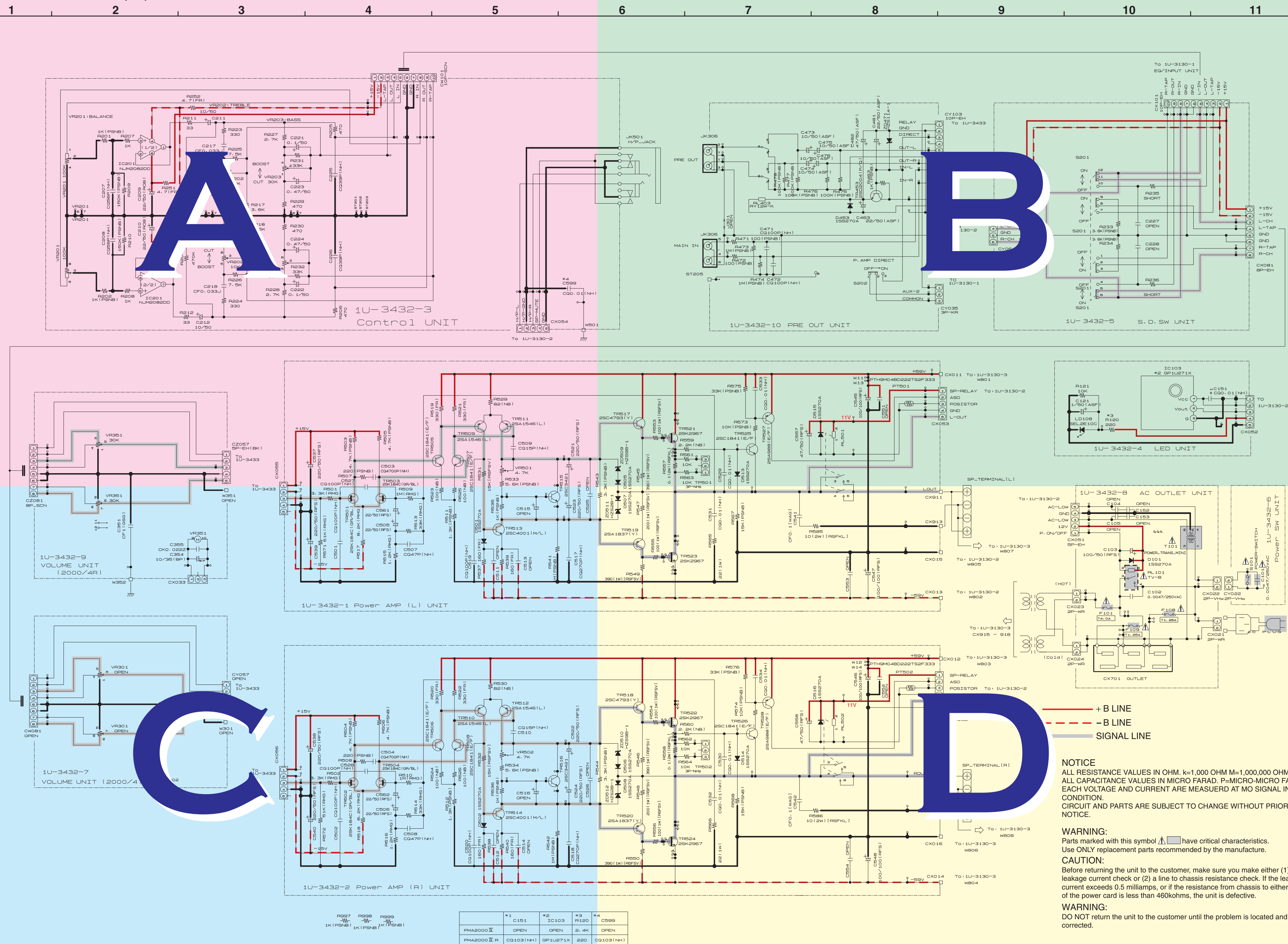
SCHEMATIC DIAGRAMS (2/3) 1U-3432 POWER AMP UNIT
