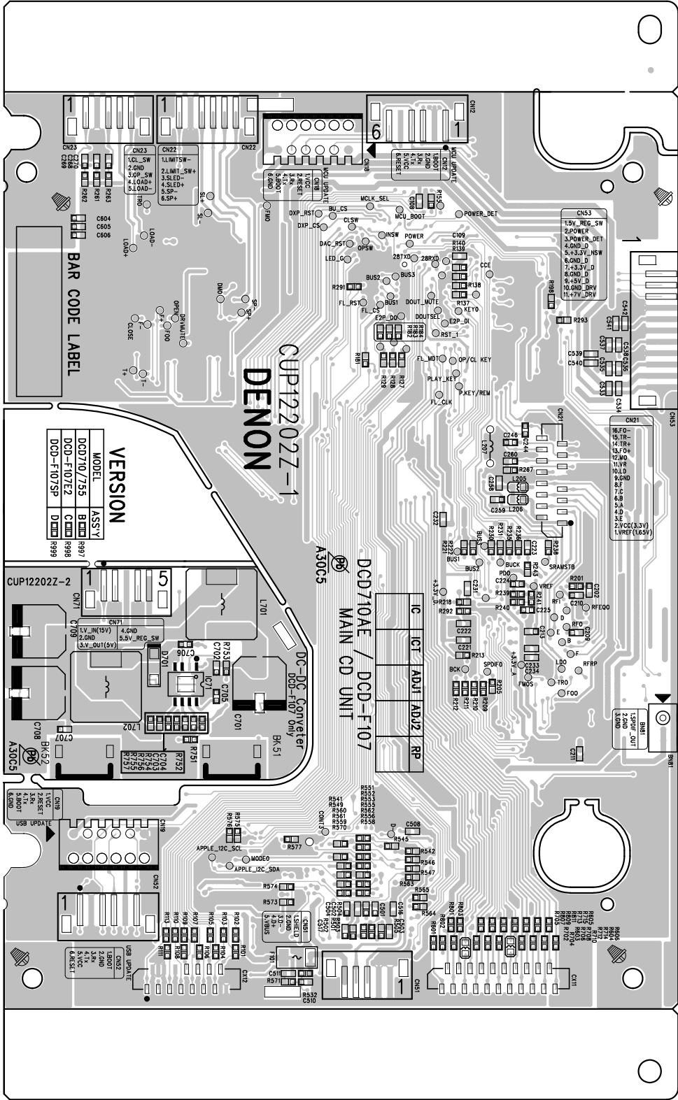
COMPONENT SIDE
