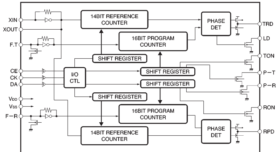
Block Diagram
