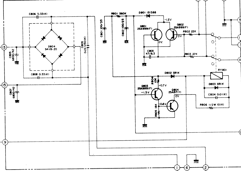
POWER SUPPLY, PROTECTOR P.C BOARD 72-1867
