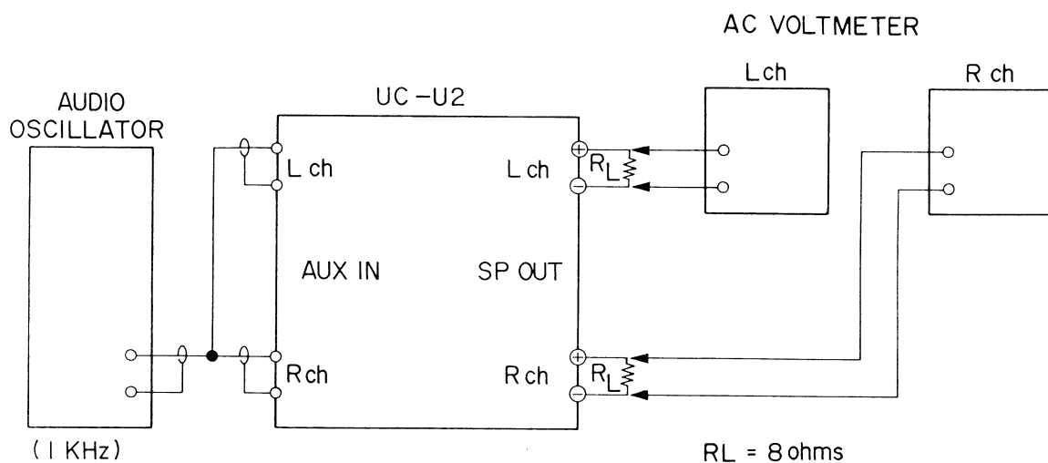
Fig. 8 Instrument Connections
