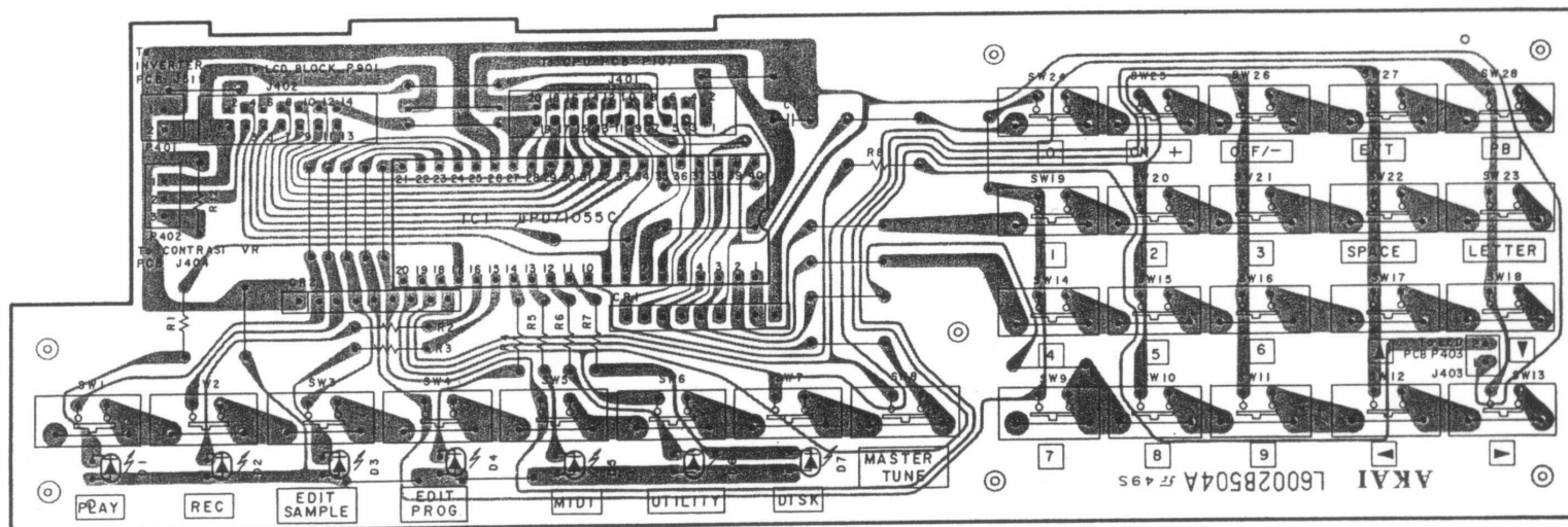
PANEL PCB L6002B504A
