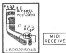
LED PCB L6002B504B
