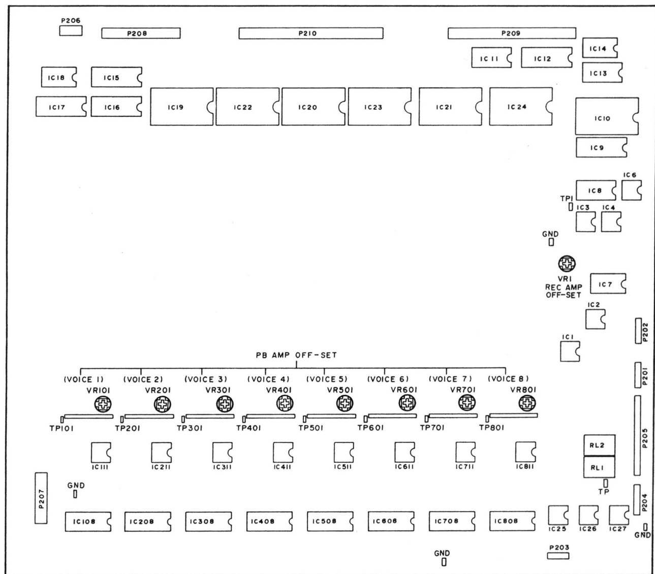
Fig. 5-1 Adjustment points of VOICE PC Board
