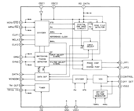
SED9420CAC (VFO TYPE FDD DATA SEPARATOR) (IC10)
