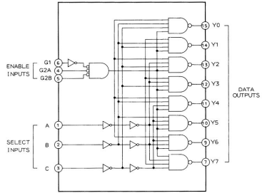
TC74HC138P [3 TO 8 DEMULTIPLEXER] (IC22 TO 24)
