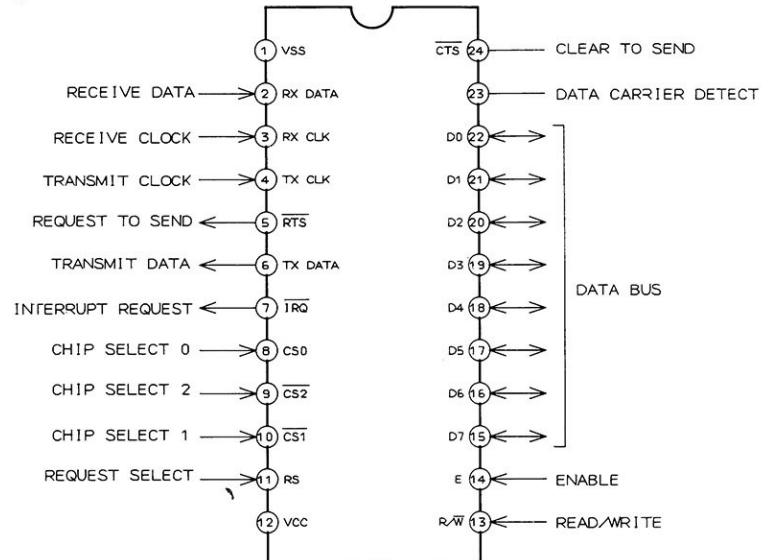
HD6850P (IC8) [COMMUNICATION INTERFACE ADAPTER]
