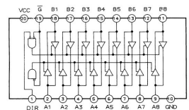
TC74HC245P [OCTAL 3 STATE TRANSCEIVER] (IC18)
