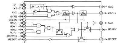
μPD71011C (CLOCK PULS GENERATOR DRIVE) (IC2)
