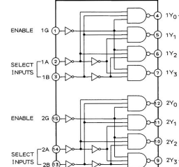
TC74HC139P [DUAL 2 TO 4 DEMULTIPLEXER] (IC29)
