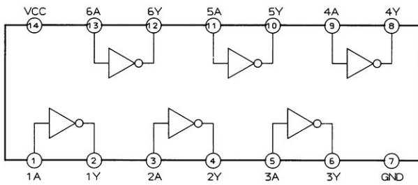
HD74LS04P (HEX INVERTER) (IC42)
