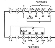
TC74HC393P (DUAL) 4-BIT BINARY COUNTER (IC19)
