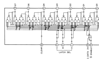
TC74HC259P [8 BIT ADABLE LATCH] (IC25)
