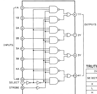
TC74HC157P [2 TO 1 DATA SELECTOR] (IC82, 89)
