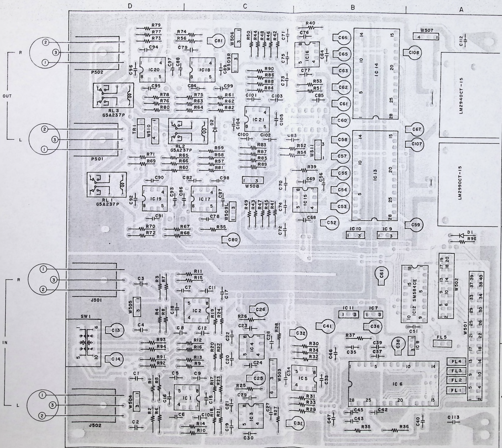
AD/DA PCB L6028A5050(J1)
