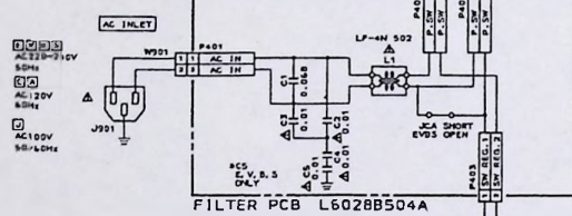
FILTER PCB L6028B504A
