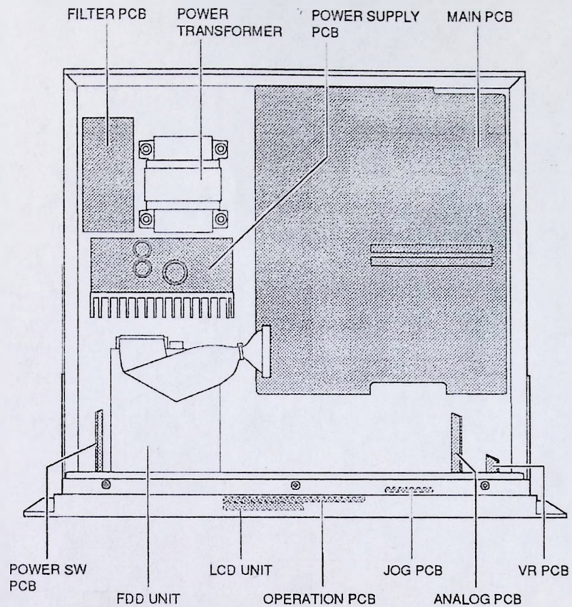
Fig. 3-1 Model S2000
