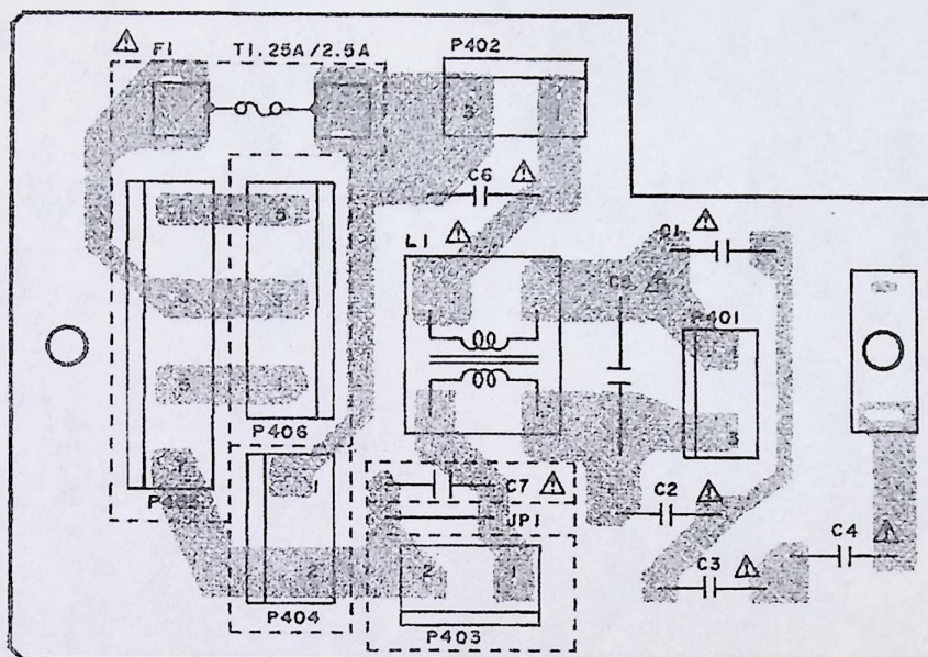
FILTER PCB L30I9B504A
