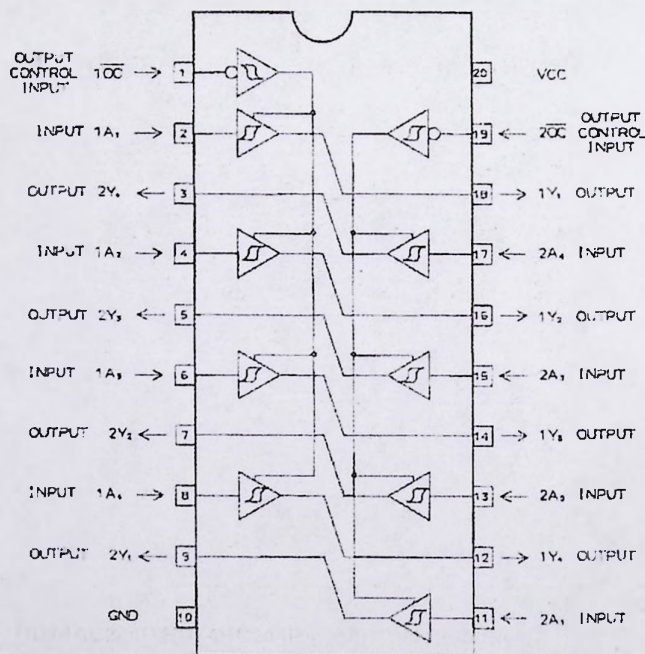
HD74AC244P/HD74HC244P (Octal 3 state buffer)
