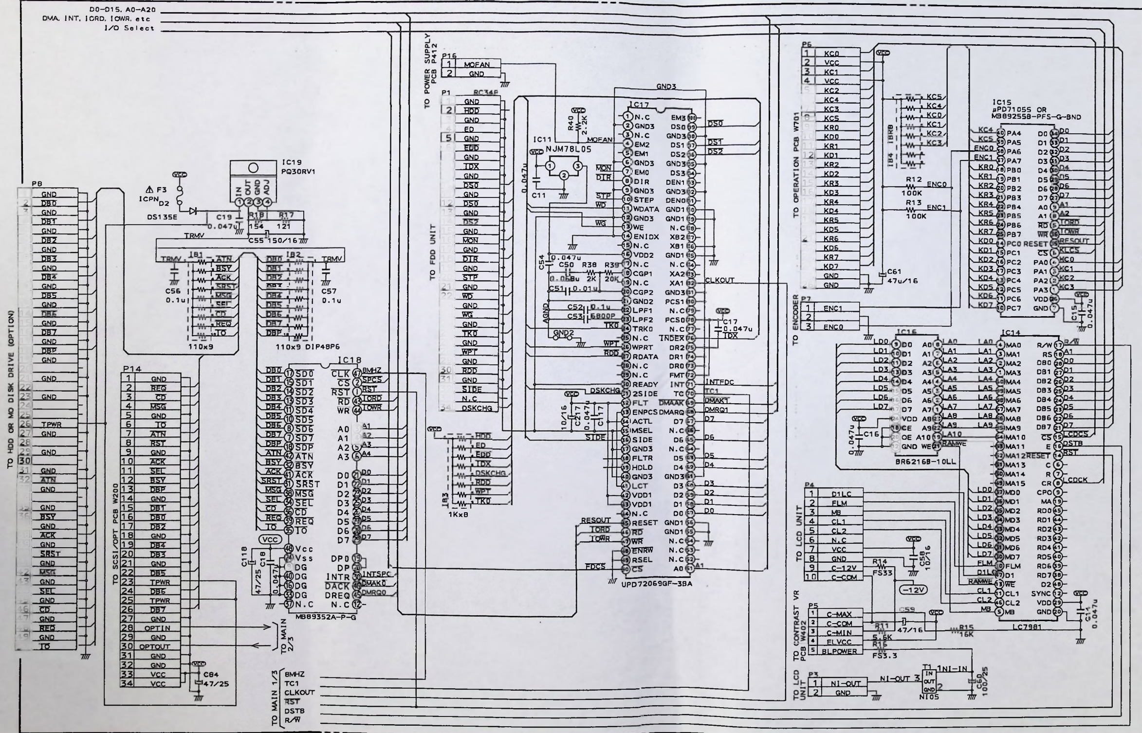
MAIN PCB L6038A502A
