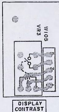
CONTRAST VR PCB L6036A502G
