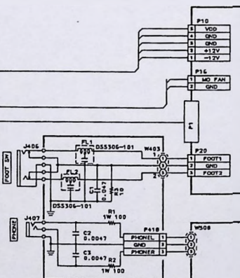
JACK(3) PCB L6028B504G
