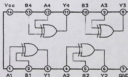
HD74HC86P (Quad exclusive OR gate)
