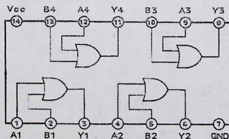
HD74HC32P (Quad 2 input OR gate)
