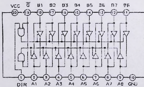
HD74HC245P (Octal 3 state transceiver)
