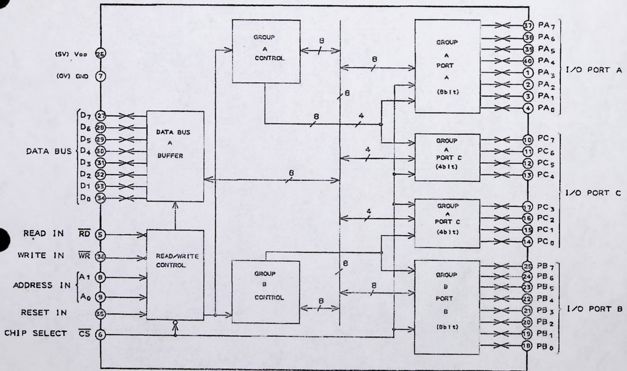
MB89255A-P-G (Parallel data I/O interface)
