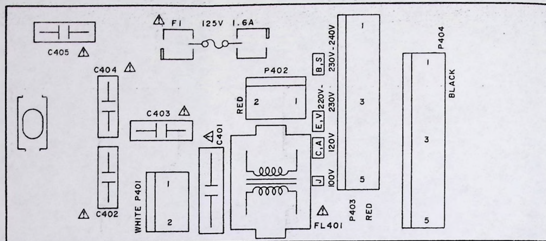
FILTER PCB L6039A503C
