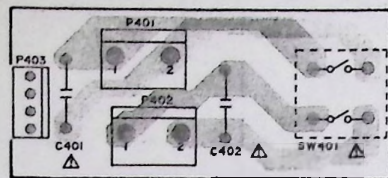
POWER SW PCB L6038A502D
