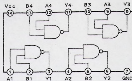
HD74HC00P (Quad 2 input NAND gate)
