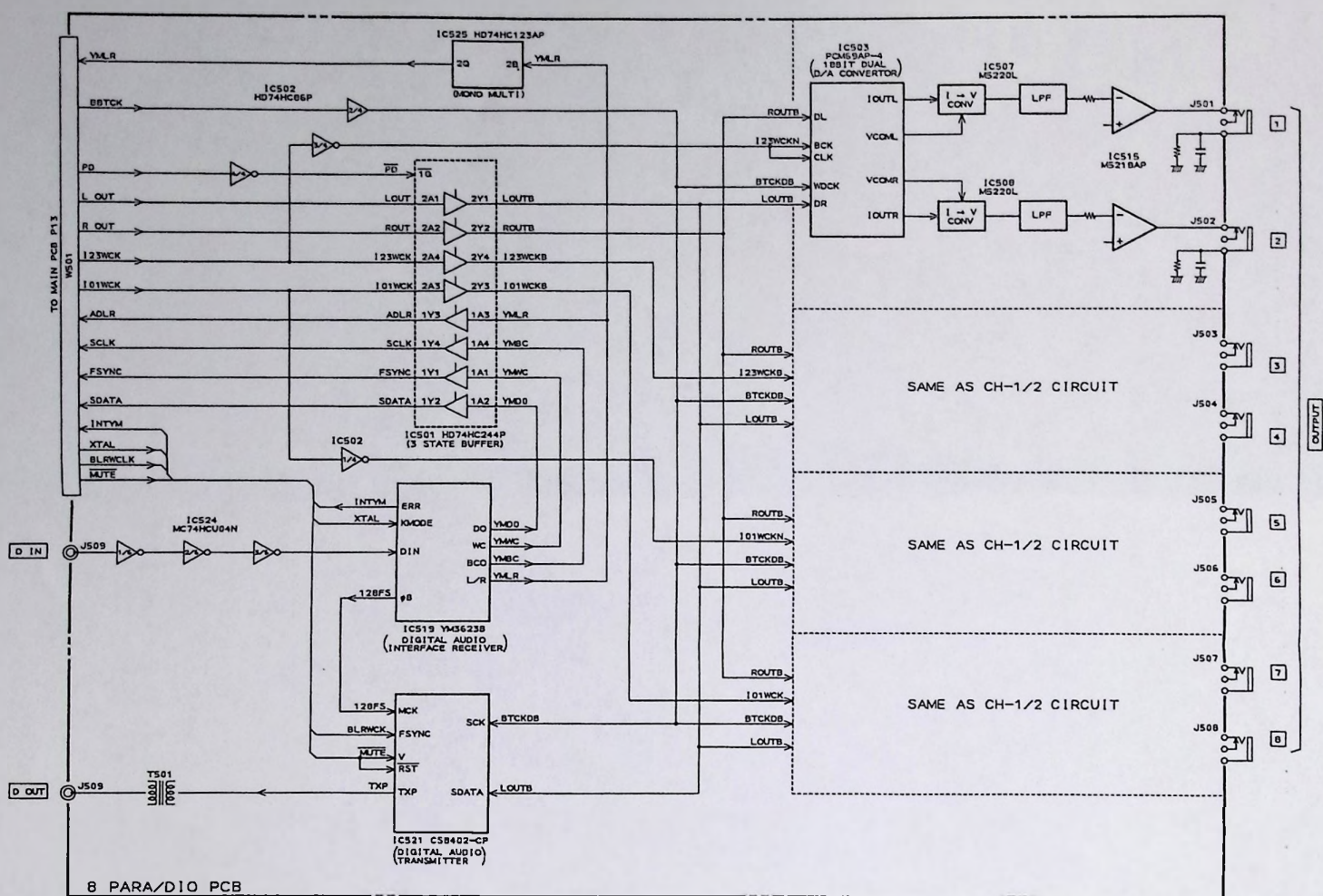
S3000XL 8 PARA/DIO (1B-208P) BLOCK DIAGRAM No.4-2 L603952M A2
