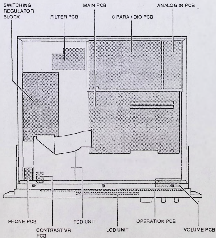
Fig. 3-2 Model S3000X1
