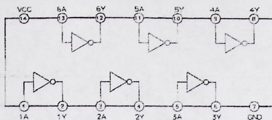
HD74AC04P/MC74HCU04N/TC74AC04P (Hex inverters)
