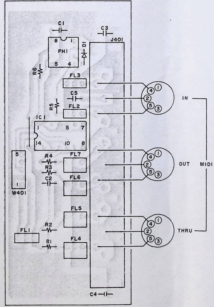
MIDI PCB L6028B504C(J1)
