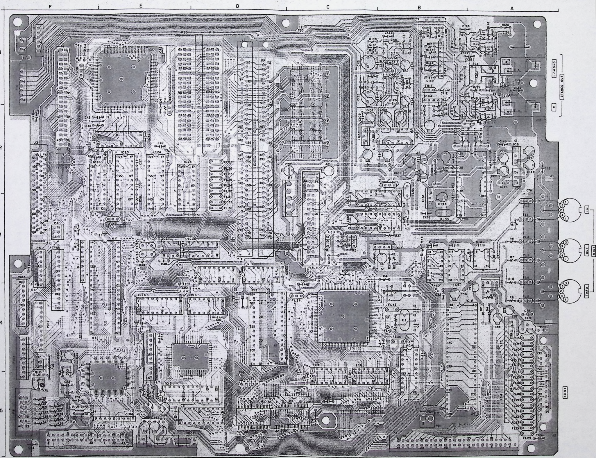
MAIN PCB L6039A5050
