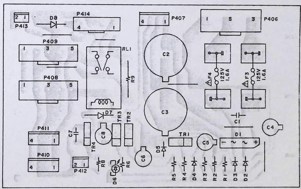
POWER SUPPLY PCB L6028B504B(J1)
