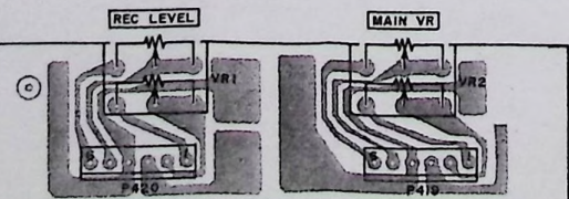
VR PCB L6028B504H(J1)
