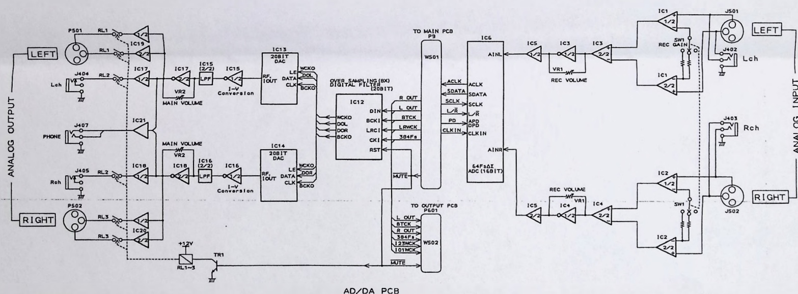
S3000XL 8 PARA/DIO (1B-208P) BLOCK DIAGRAM No.4-2 L603952M A2
