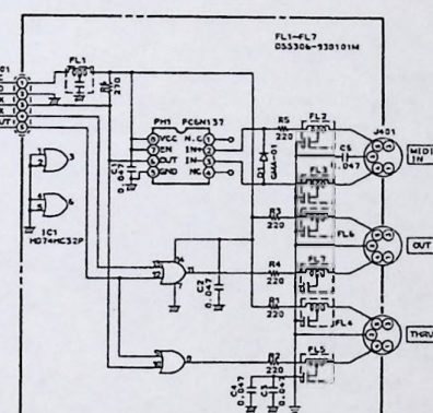
MIDI PCB L6028B504C
