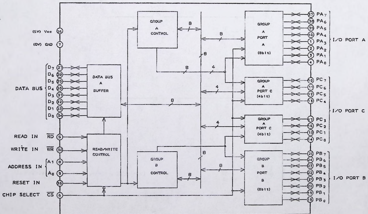
MB89255A-P-G (Parallel data I/O interface)
