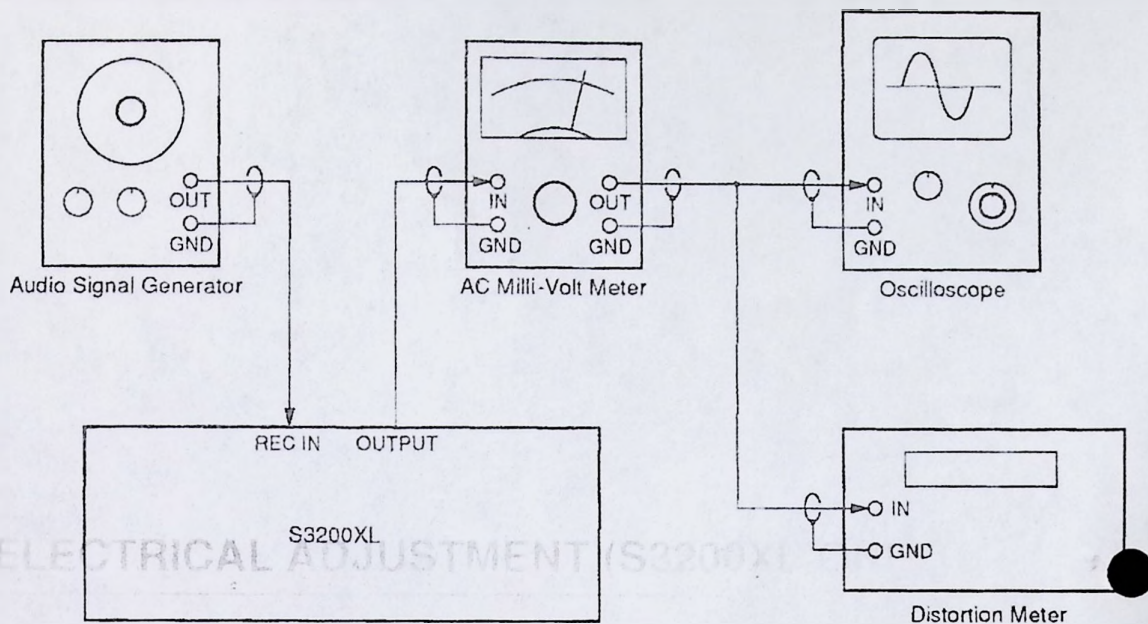
Fig. 4-1 Instrument connection
