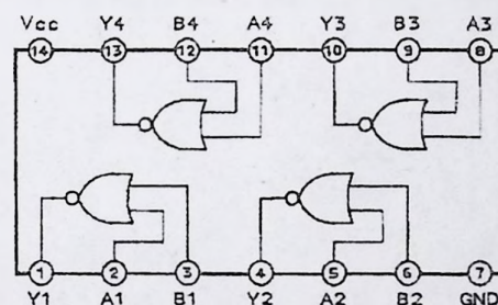
HD74HC02P (Quad 2 input NOR gate)
