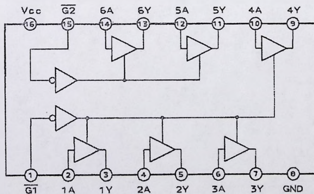
HD74HC367P (Hex 3-state bus buffers)
