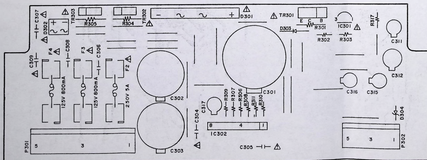
POWER SUPPLY PCB L6039A503B
