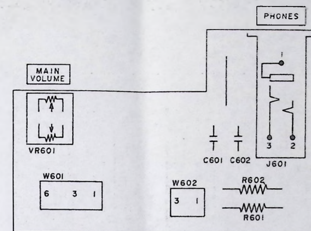
VR PCB L6039A503E
