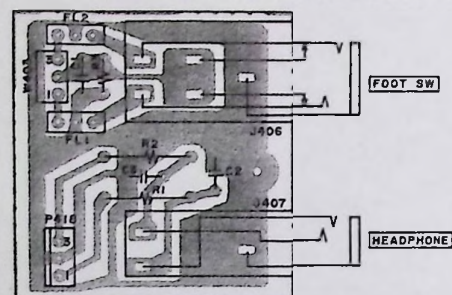
JACK(3) PCB L6028B504G(J1)
