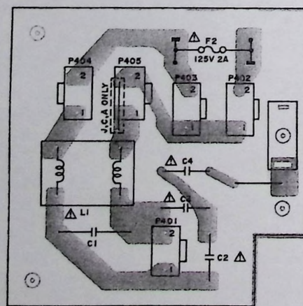
FILTER PCB L6028B504A(J1)
