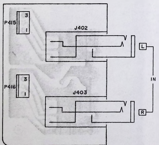
JACK(1) PCB L6028B504E(J1)
