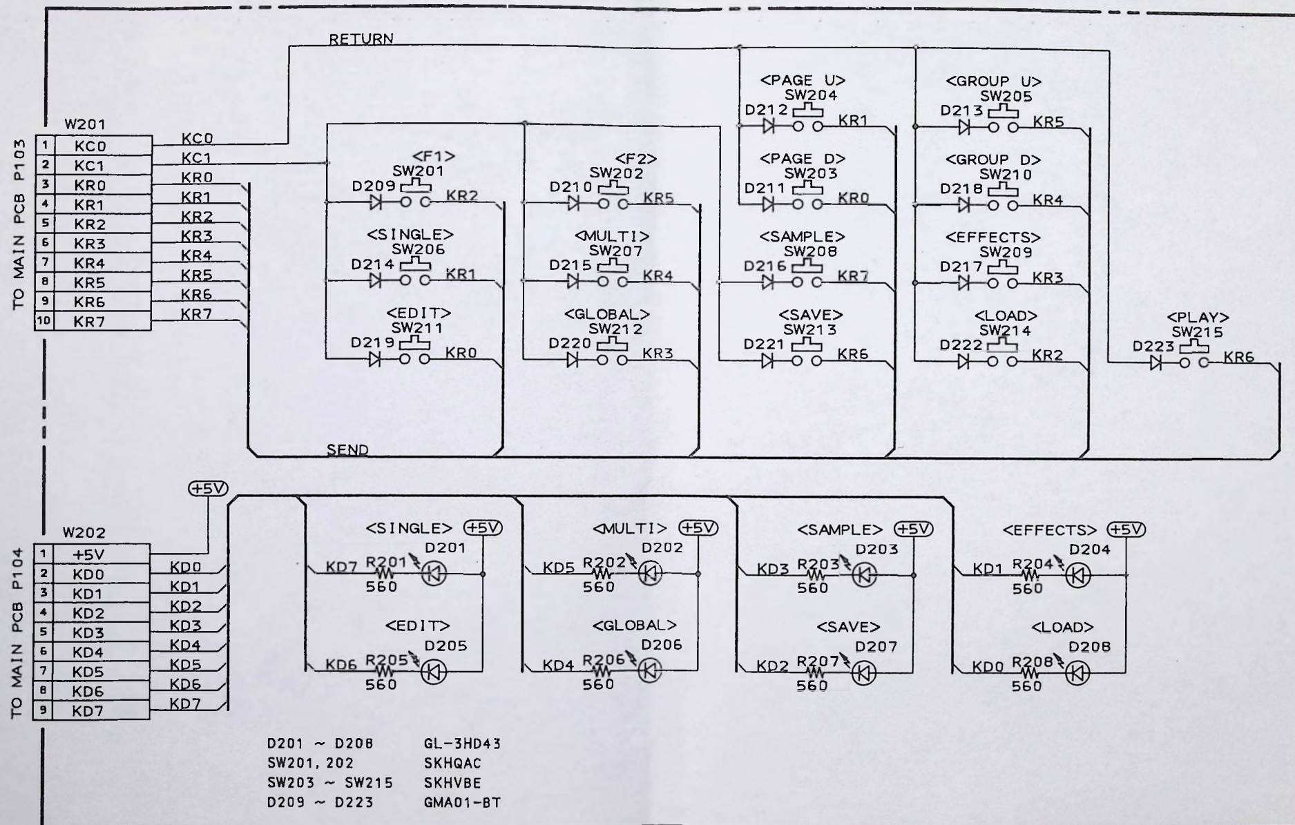
OPERATION PCB L6039A503A
