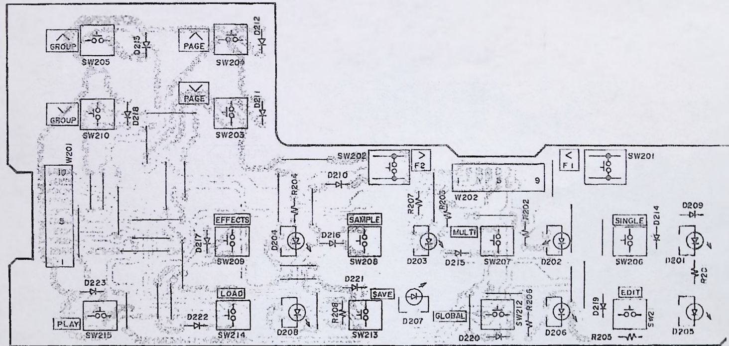
OPERATION PCB L6039A503A
