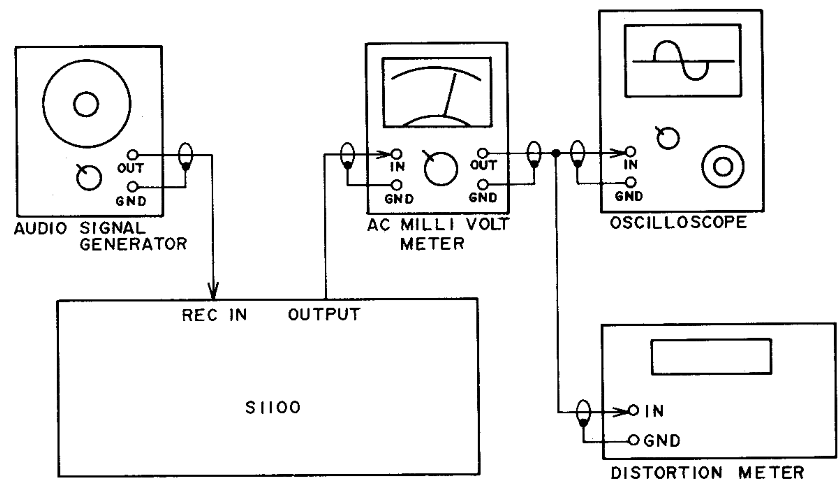
Fig. 3-1 Instrument connection
