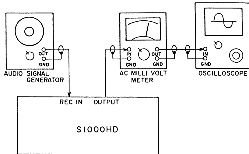
Fig. 4-1 Instrument connection
