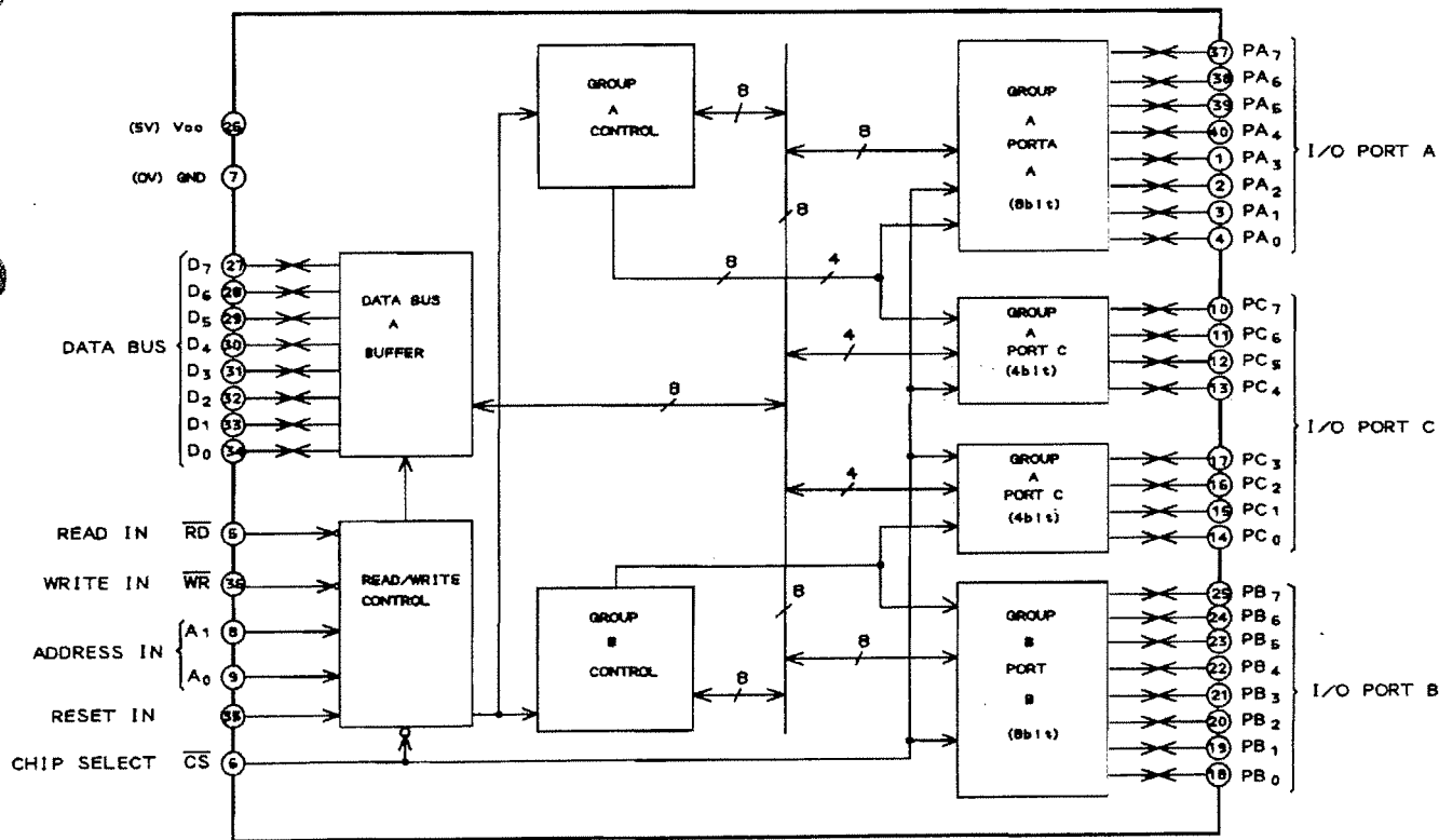
MB89255B-P-G (Parallel data I/O interface)
