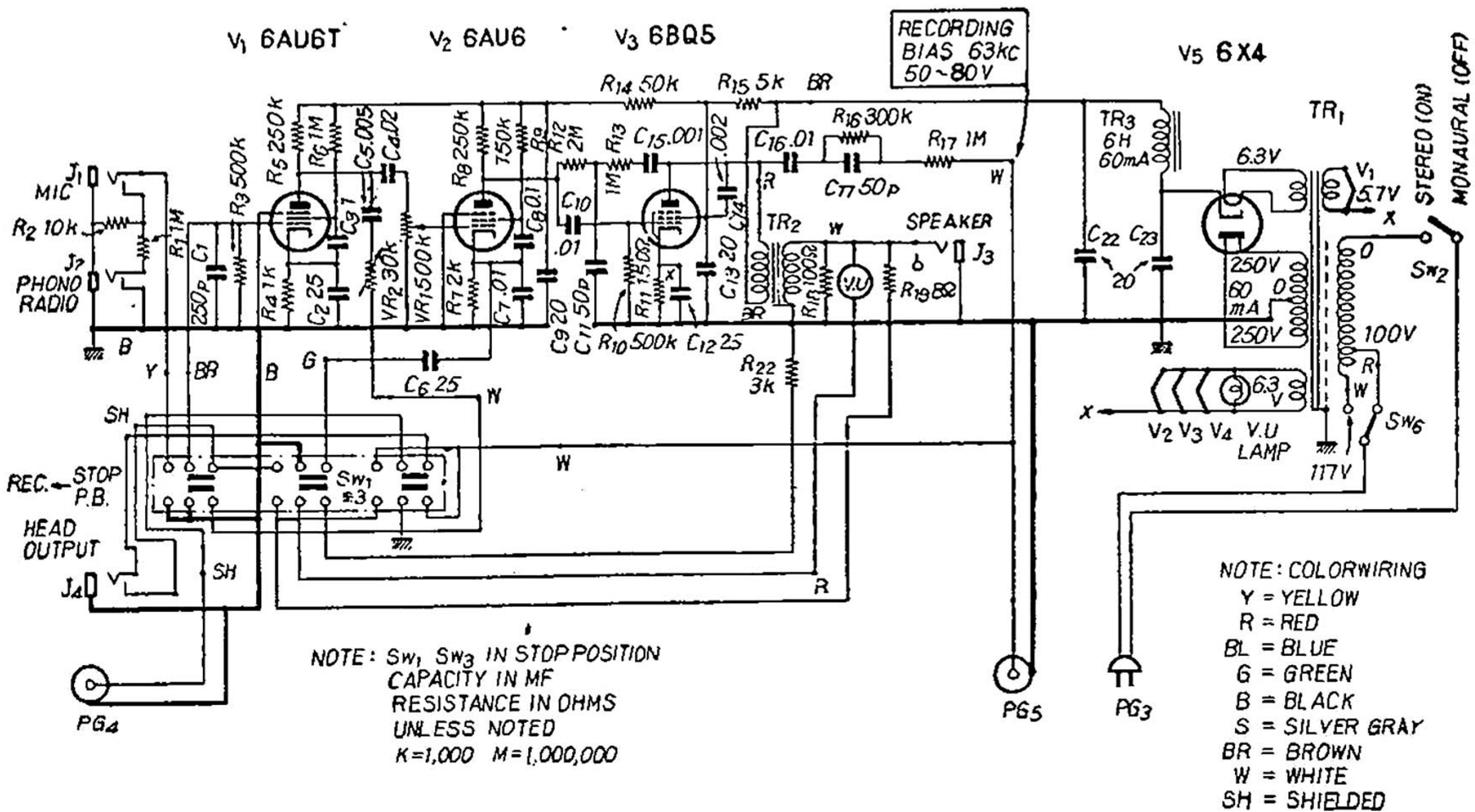
AKAI TEREORDER MULTI-FOUR SCHEMATIC AKAI ELECTRIC CO. LTD.
