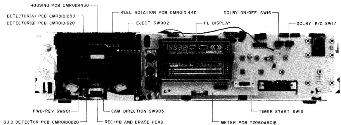
Fig. 4-1 Front View
