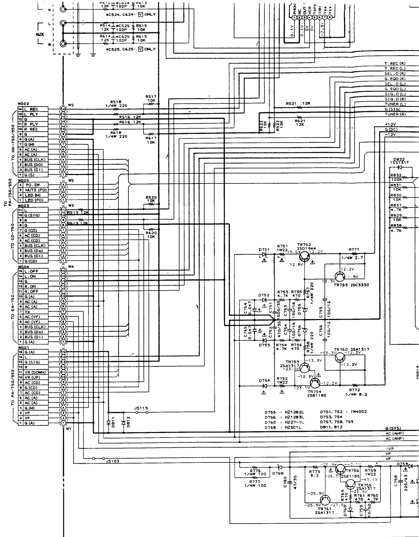
CONTROL PCB A6007A502B
