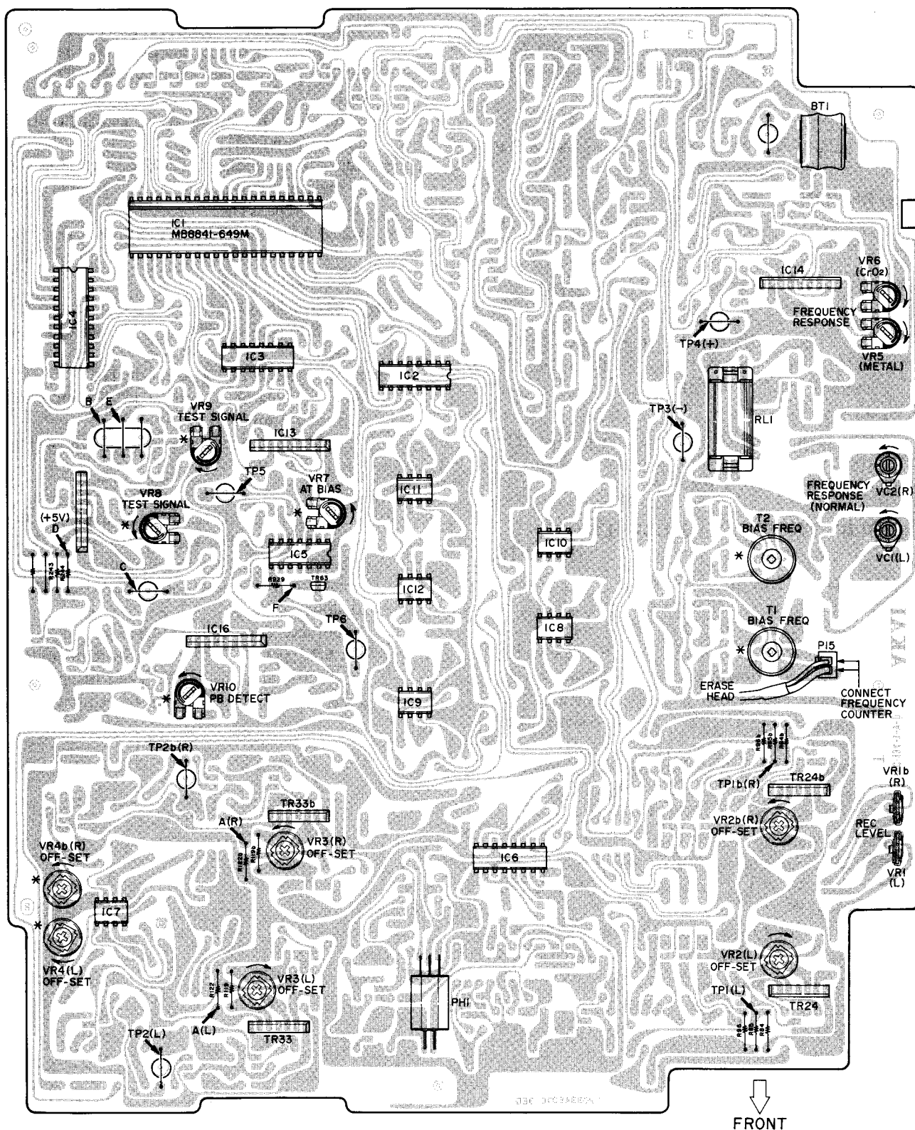
Fig. 2-17 Tuning PCB (Parts Side View)
