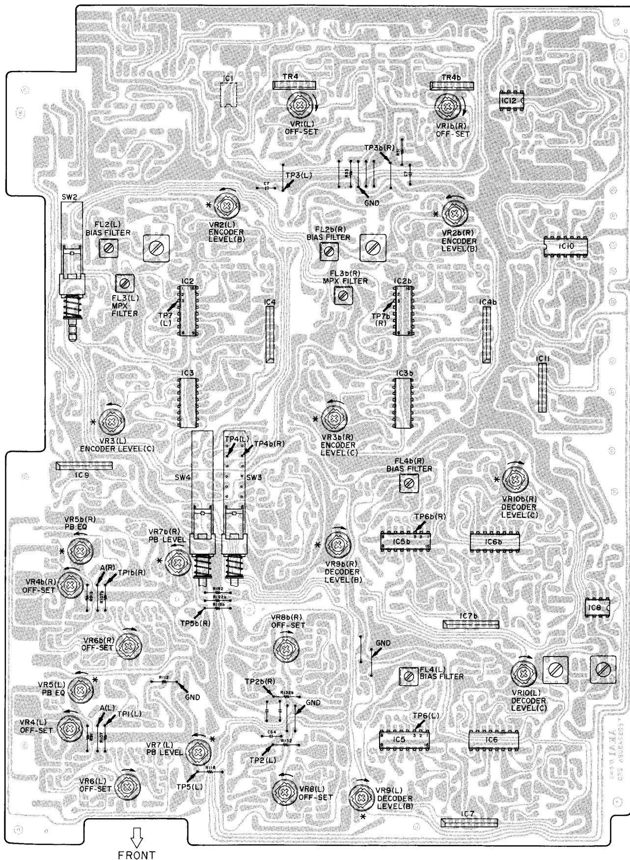
Fig. 2-16 Pre Amp PCB (Parts Side View)
