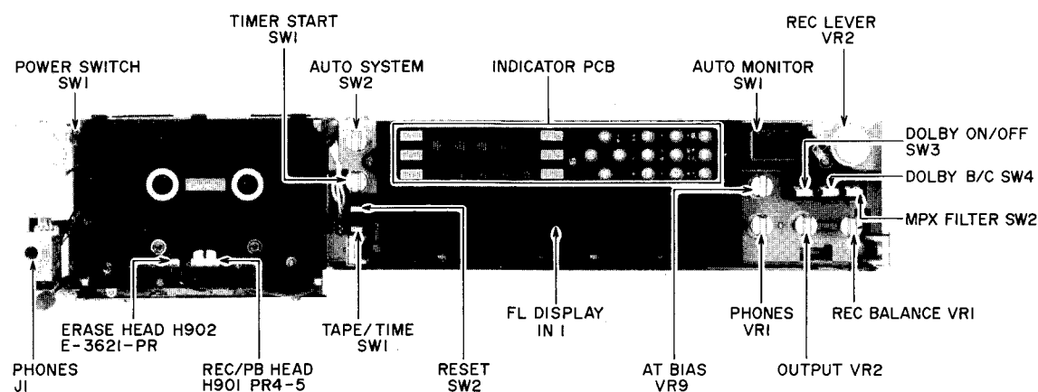
Fig. 2-5 Front View
