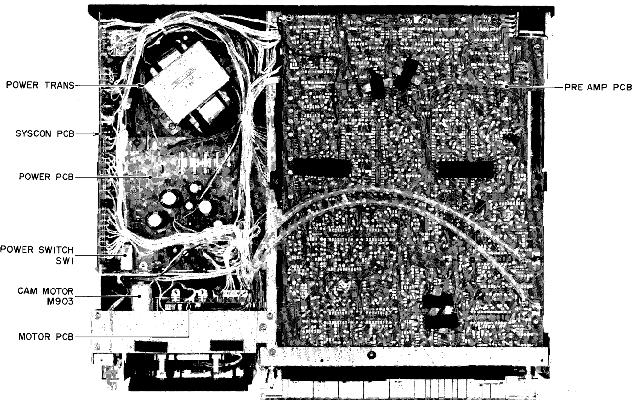
Fig. 2-6 Top View
