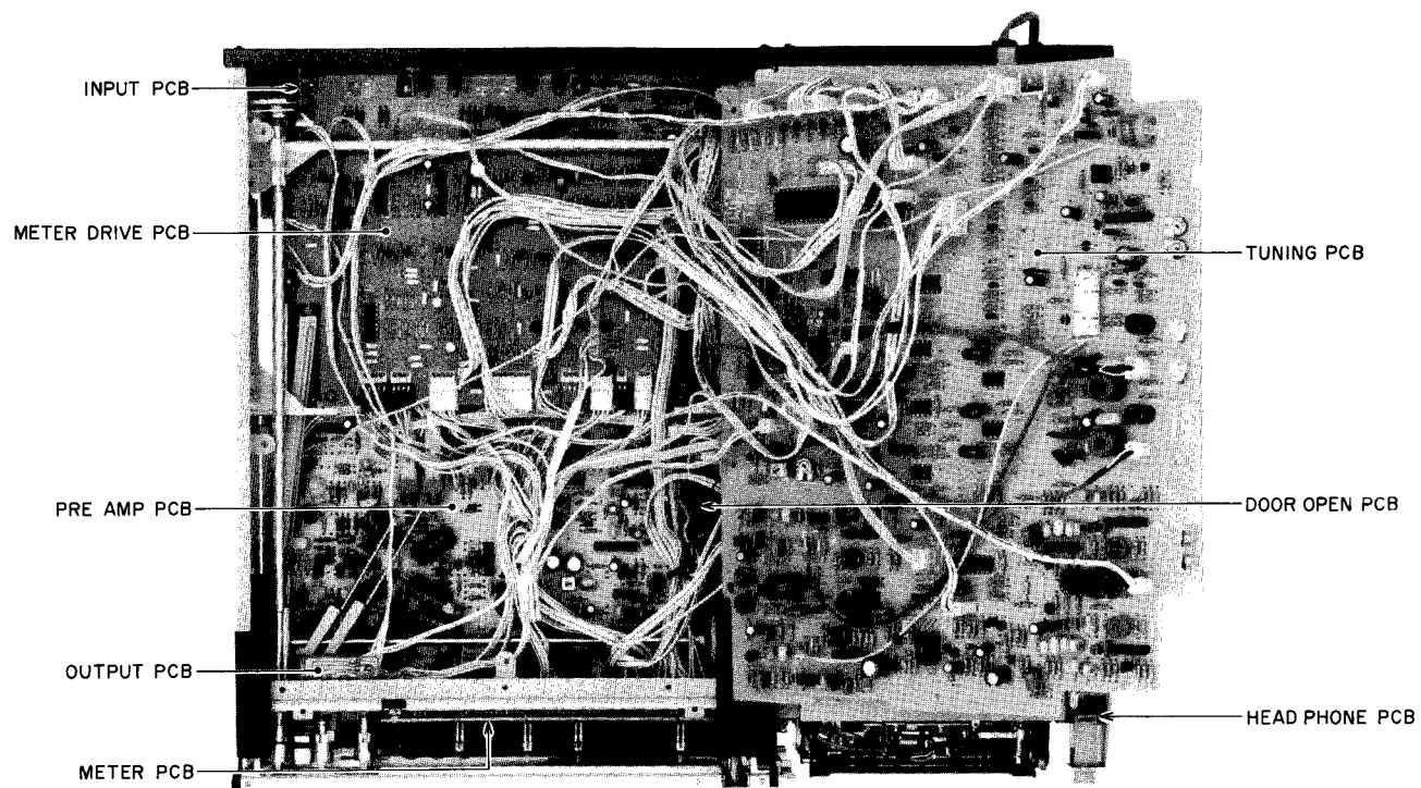
Fig. 2-7 Bottom View
