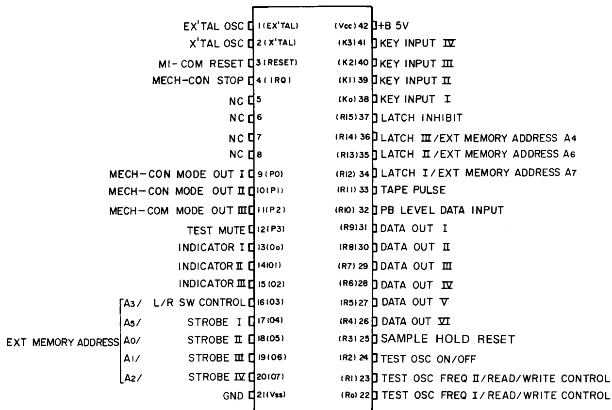
Fig. 1-4 IC1 MB8841-649M
