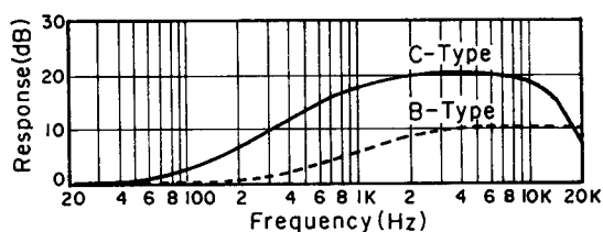
Fig. 15 Encode Characteristics of Dolby B-type and C-type in low level
