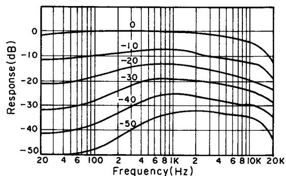
Fig. 14 Encode Characteristic of Dolby C-type NR
