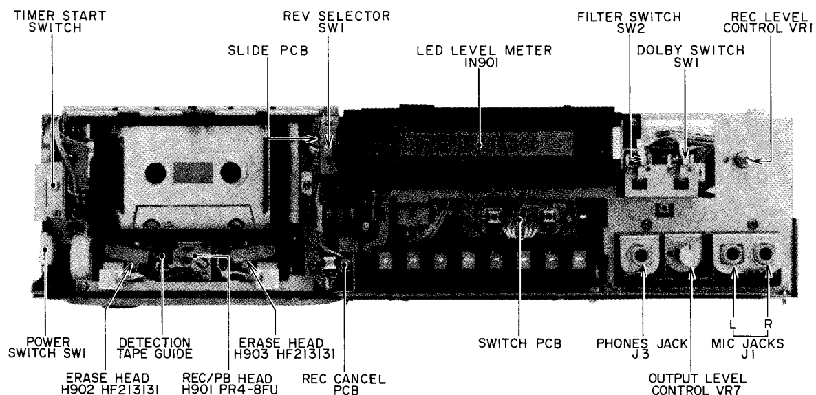
Fig. 2 Front View
