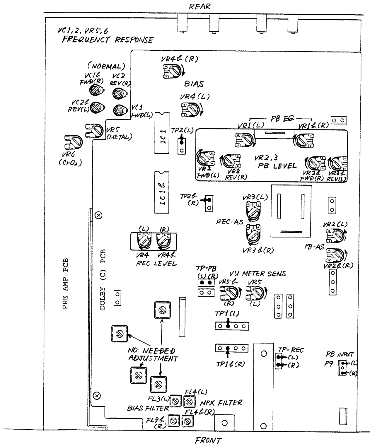
Fig. 4 Amplifier Adjustment
