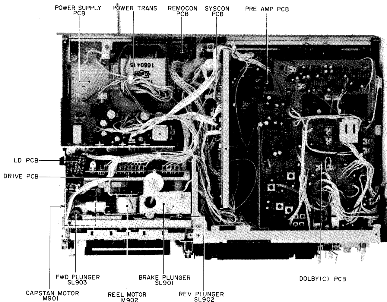
Fig. 3 Top View
