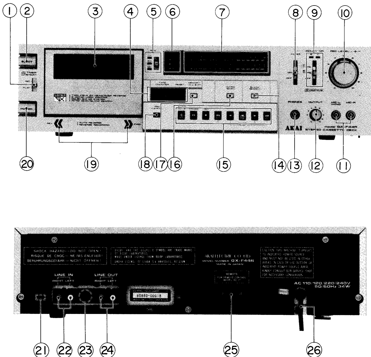
Fig. 1 Controls
