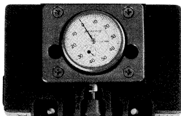
Fig. 20 AKAI Head Projection Gauge (TF-111CJ)
