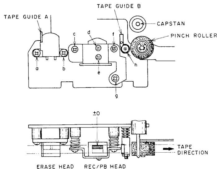
Fig. 9 Head Adjustment
