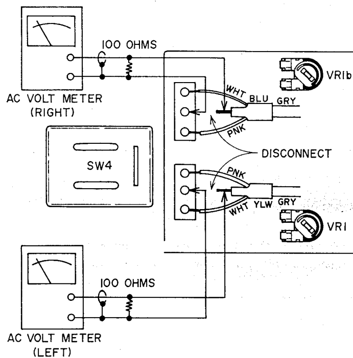
Fig. 13 Rec Peaking
