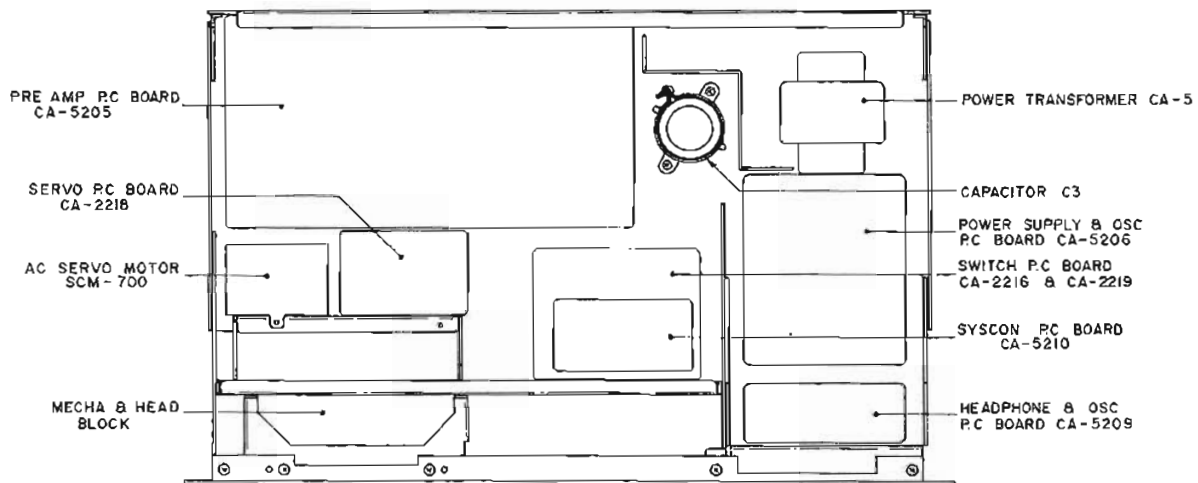
Fig. 2 Top View
