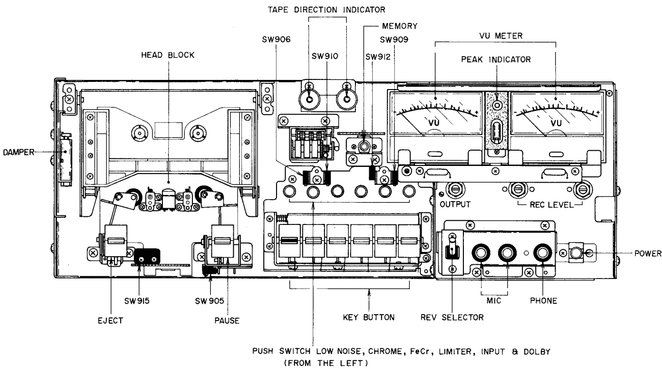
Fig. 2 Front View
