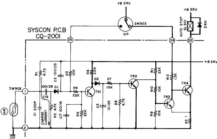
SCHEMATIC-11
