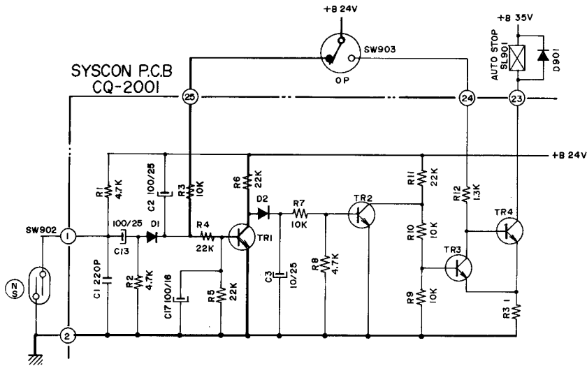
SCHEMATIC-8
