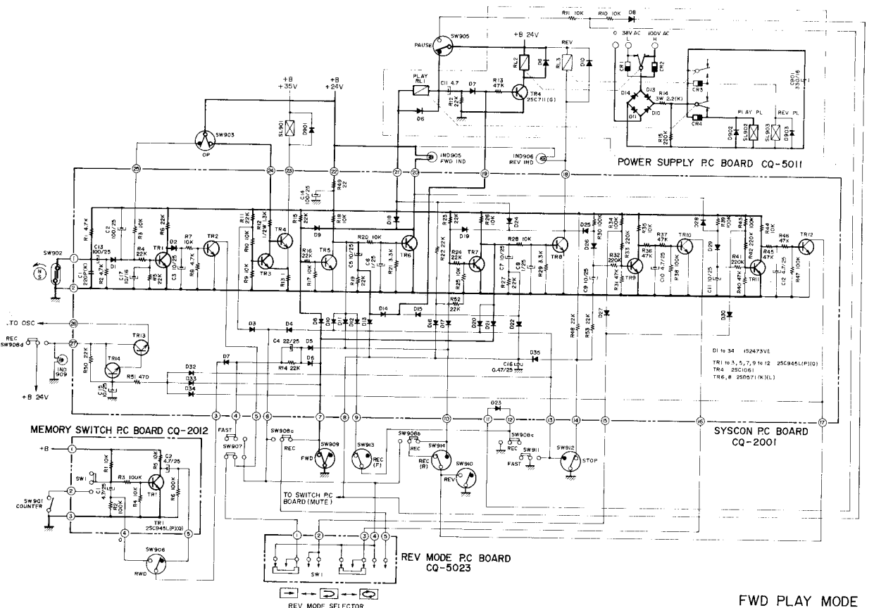
SCHEMATIC-2
