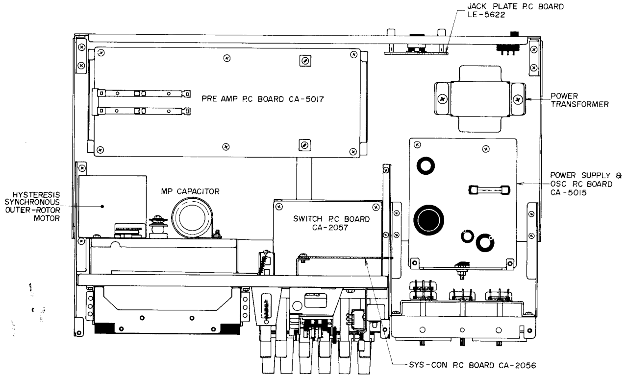
TOP VIEW
