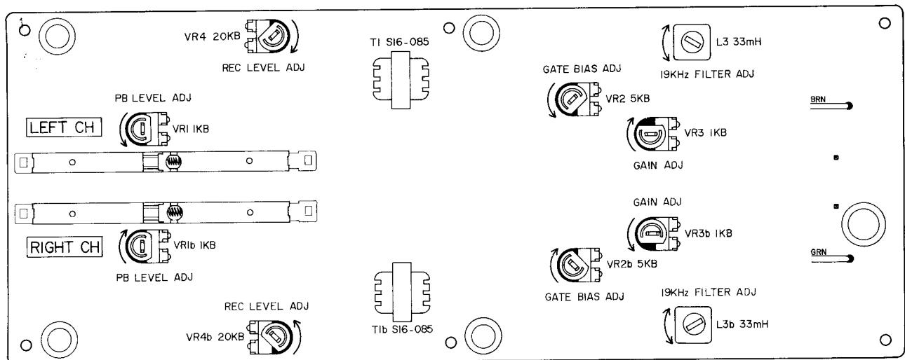
Fig. 9 Pre Amp P.C Board CA-5017
